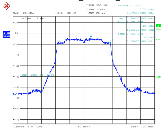
802.11ax40_5670MHz_Chain 0
