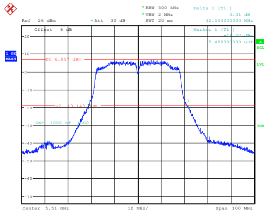
802.11ac40_5510MHz_Chain 1
