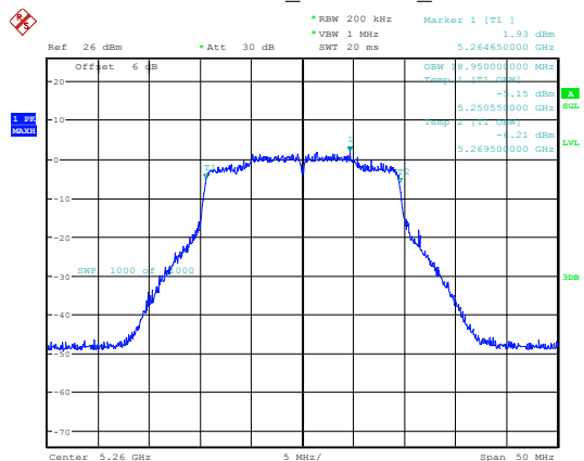
802.11ax20_5260MHz_Chain 0
