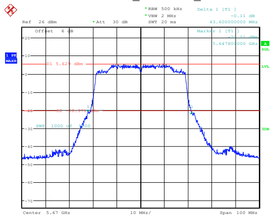
802.11ax40_5670MHz_Chain 0
