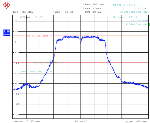
802.11ac40_5550MHz_Chain 1
