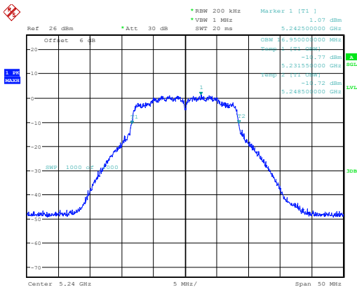
802.11a_5240MHz_Chain 1
