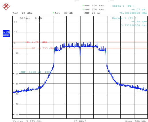
802.11ac80_5775MHz_Chain 0
