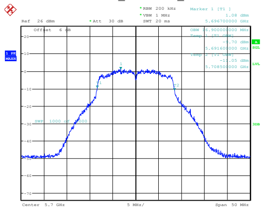
802.11a_5700MHz_Chain 1
