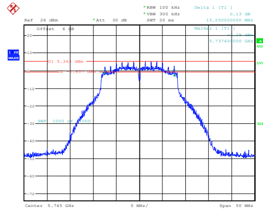
802.11a_5745MHz_Chain 1
