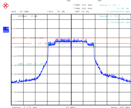
802.11ac80_5775MHz_Chain 1
