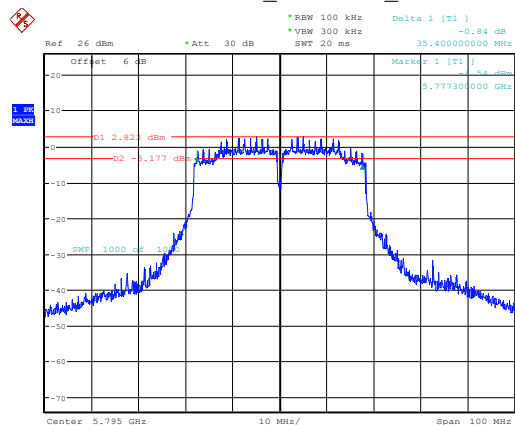
802.11ac40_5795MHz_Chain 0
