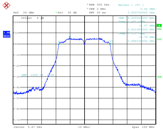
802.11ac40_5670MHz_Chain 0
