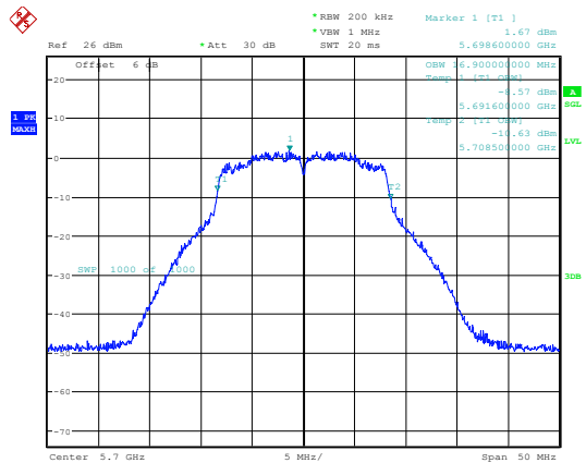
802.11a_5700MHz_Chain 0
