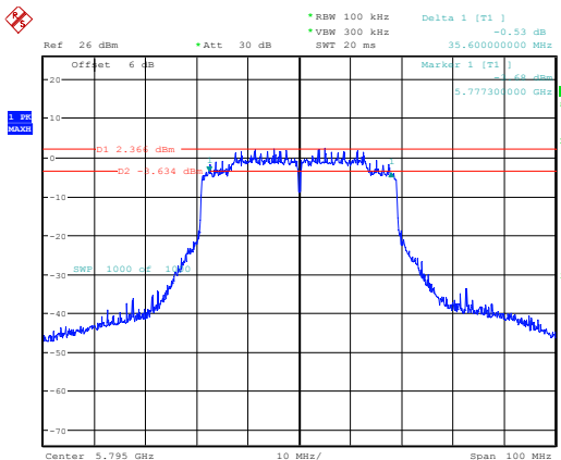
802.11ax40_5795MHz_Chain 0
