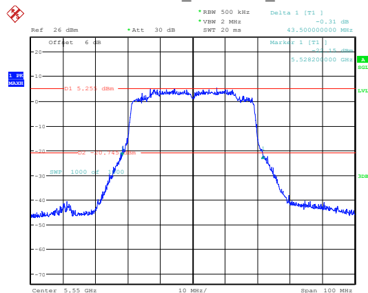
802.11ax40_5550MHz_Chain 1
