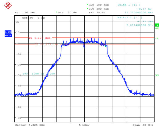
802.11a_5825MHz_Chain 1
