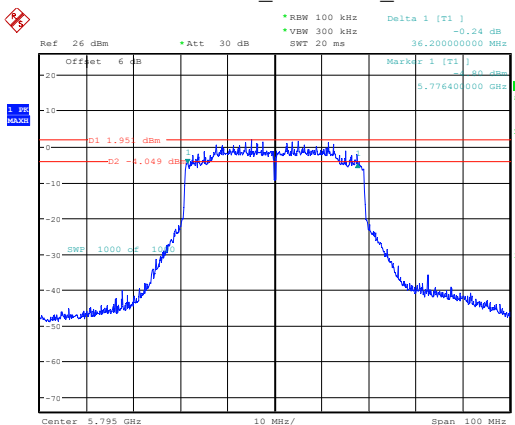
802.11ax40_5795MHz_Chain 1
