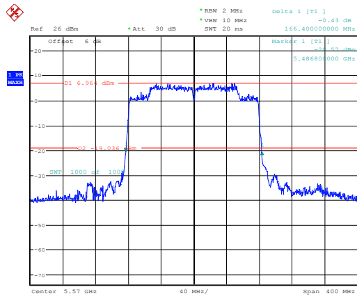
802.11ax160_5570MHz_Chain 0
