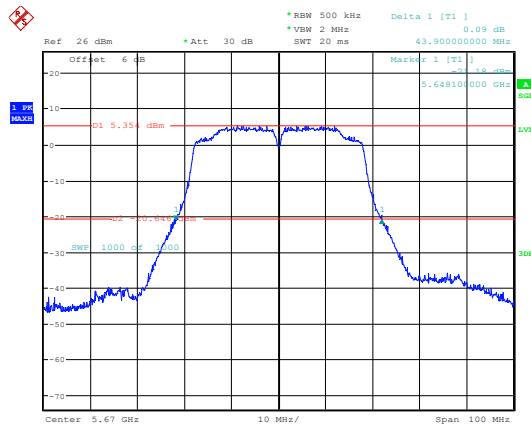
802.11ac40_5670MHz_Chain 0
