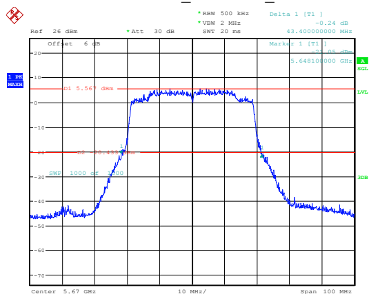
802.11ax40_5670MHz_Chain 1
