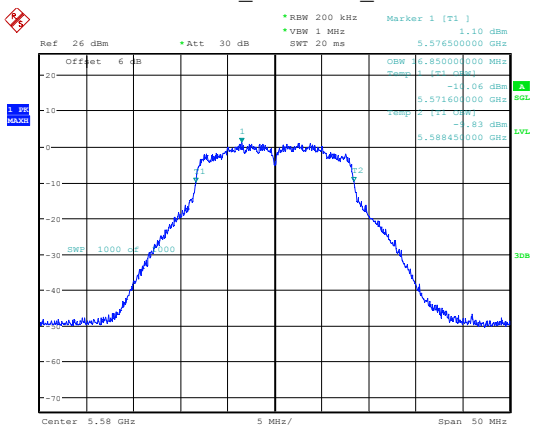
802.11a_5580MHz_Chain 1
