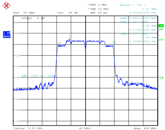
802.11ac160_5250MHz_Chain 0
