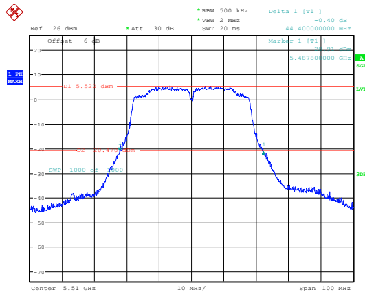
802.11ac40_5510MHz_Chain 0
