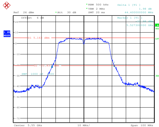
802.11ac40_5550MHz_Chain 0
