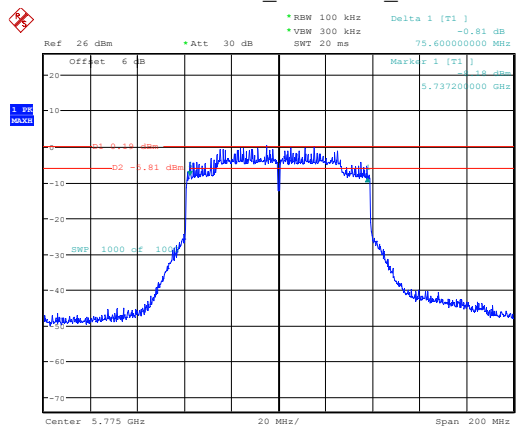
802.11ax80_5775MHz_Chain 0
