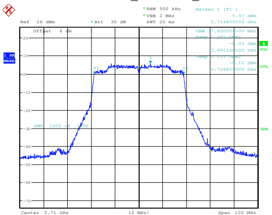
802.11ax40_5710MHz_Chain 0
