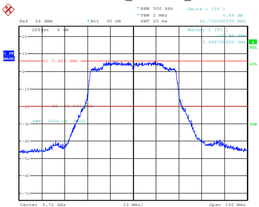
802.11ax40_5710MHz_Chain 0
