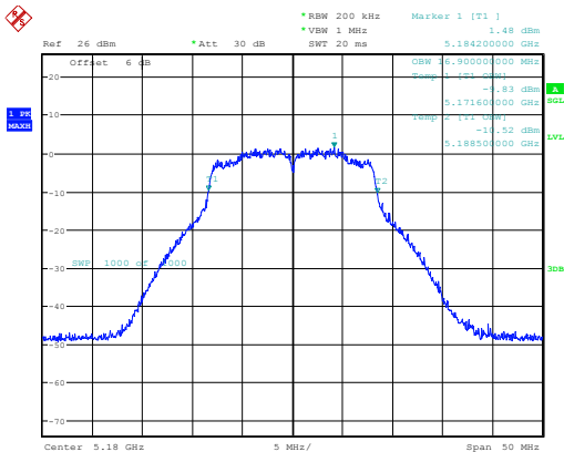
802.11a_5180MHz_Chain 1
