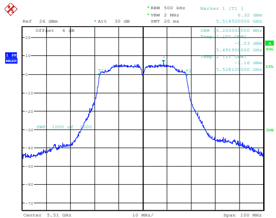
802.11ac40_5510MHz_Chain 0
