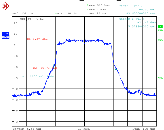
802.11ax40_5550MHz_Chain 0
