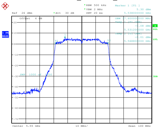
802.11ax40_5550MHz_Chain 0
