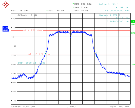
802.11ac40_5670MHz_Chain 1
