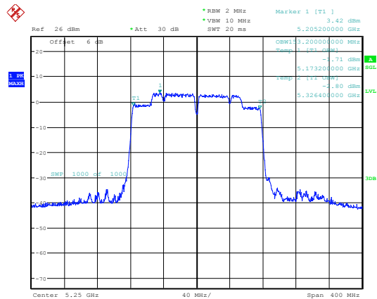
802.11ac160_5250MHz_Chain 1
