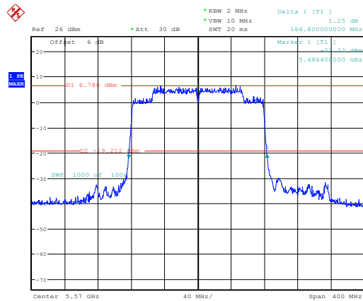
802.11ax160_5570MHz_Chain 1
