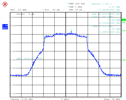
802.11ax20_5280MHz_Chain 1
