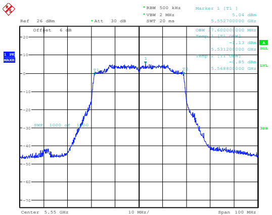
802.11ax40_5550MHz_Chain 1
