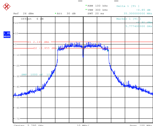
802.11ac40_5795MHz_Chain 1
