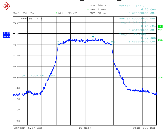
802.11ax40_5670MHz_Chain 1
