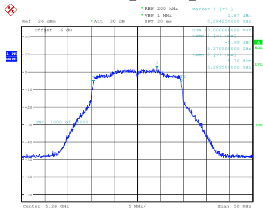
802.11ax20_5280MHz_Chain 0
