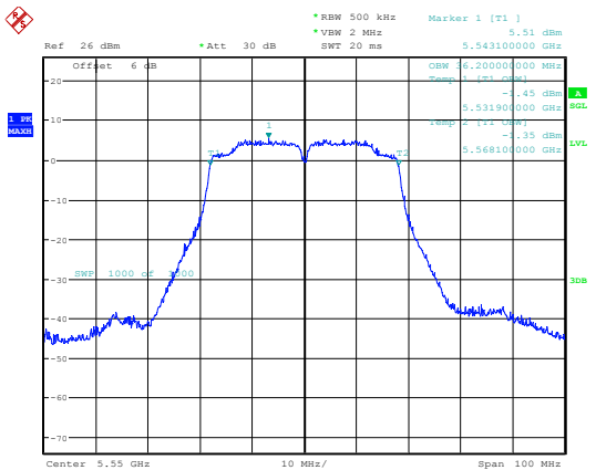
802.11ac40_5550MHz_Chain 0
