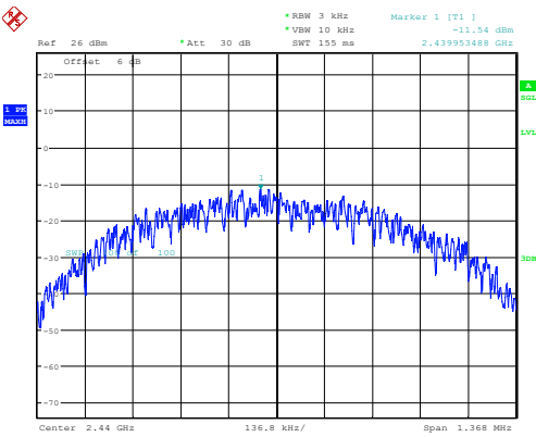
BLE_1M_Middle_Channel
