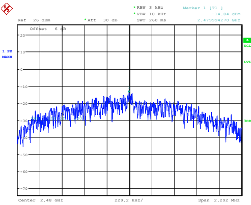
BLE_2M_High_Channel
