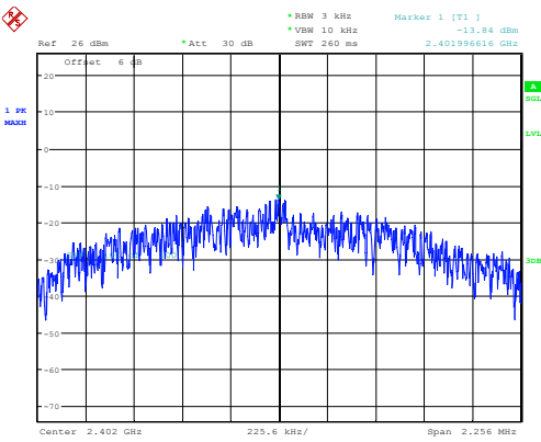
BLE_2M_Low_Channel
