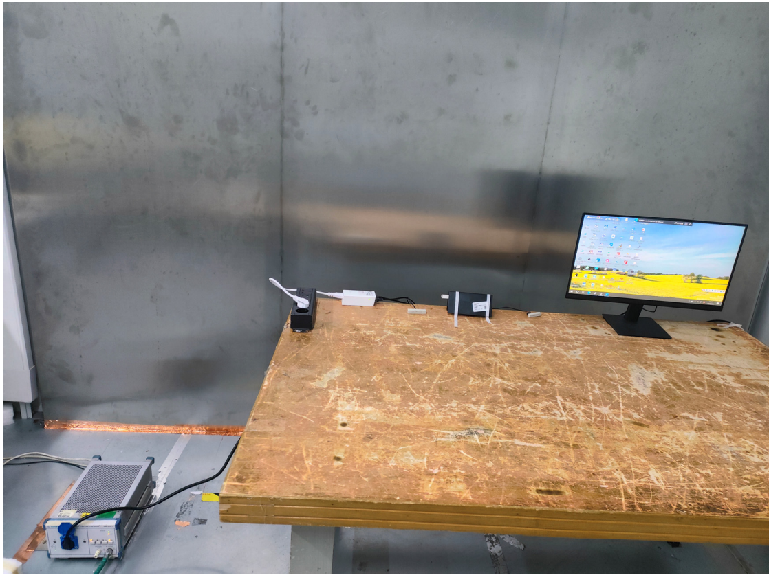
Conducted Emissions - Front View (For POE)
