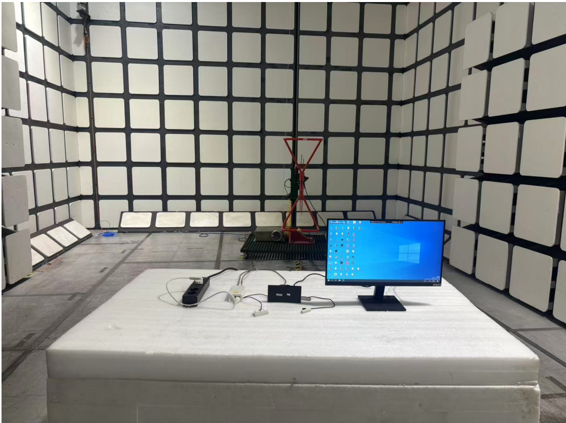
Radiated Emissions View (Below 1 GHz) (For POE)
