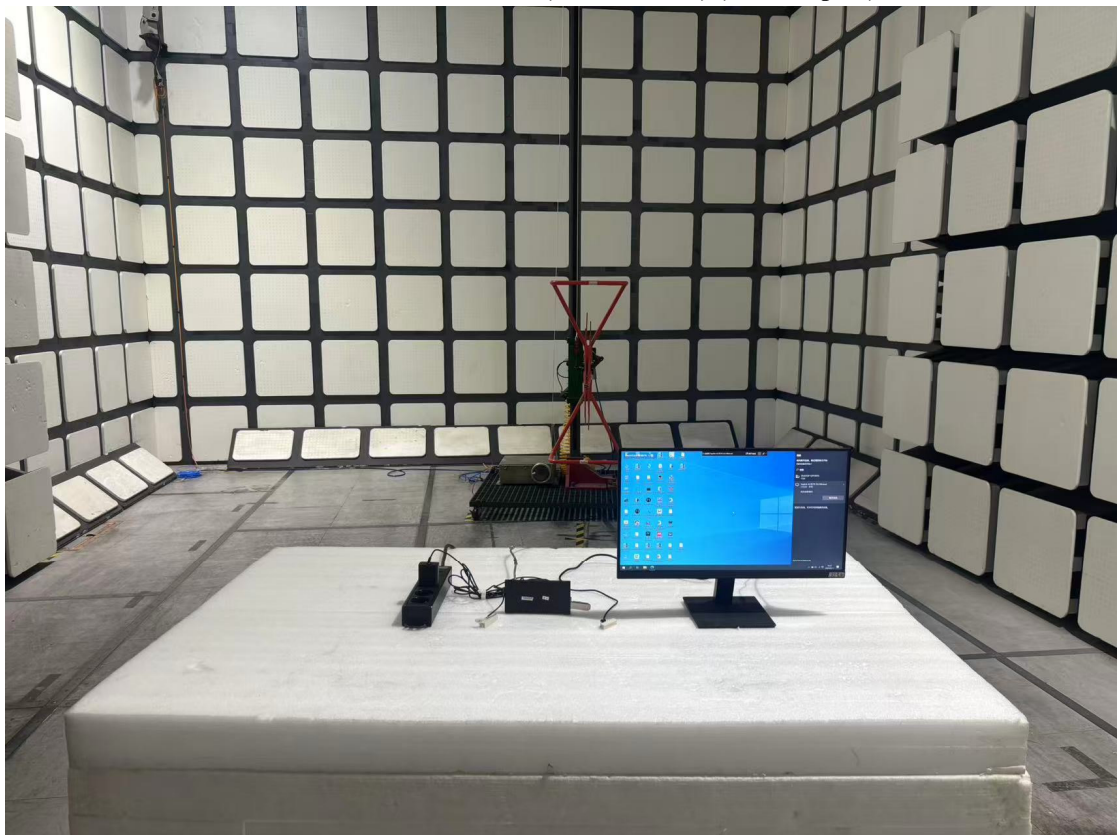
Radiated Emissions View (Below 1 GHz) (For Adapter)
