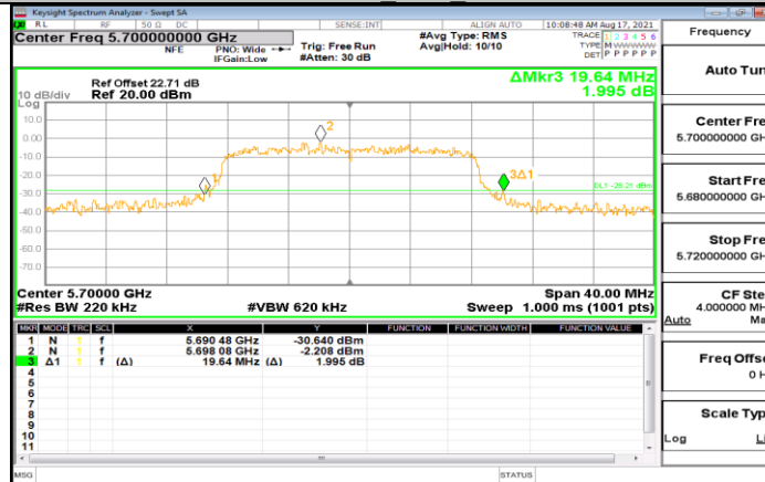
11A-CDD Ant2 5700
