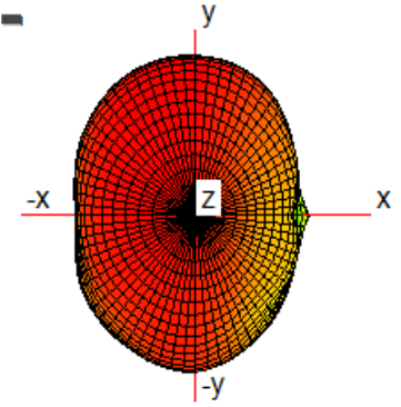
3D Antenna pattern
