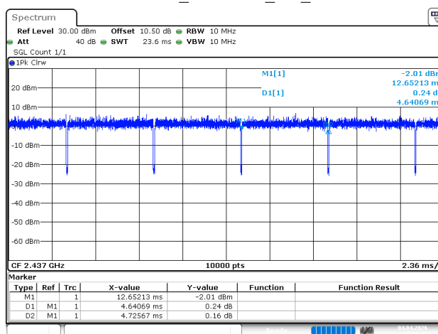
802.11ax20_2437MHz_RU_FULL
