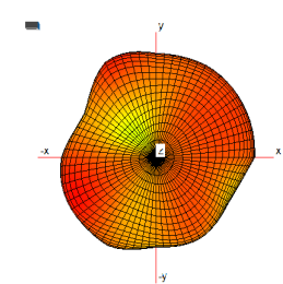
2442MHz 3D Antenna Graph
