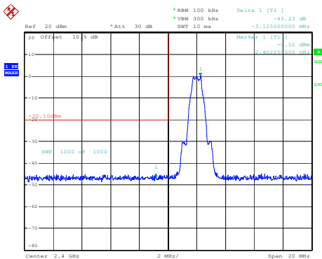
BLE_1M_Low_Channel
