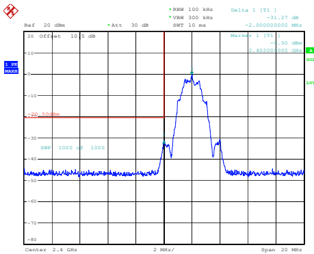
BLE_2M_Low_Channel
