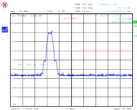
BLE_1M_High_Channel
