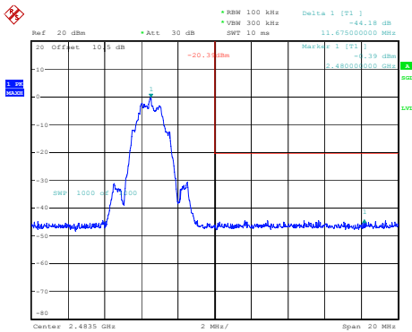
BLE_2M_High_Channel
