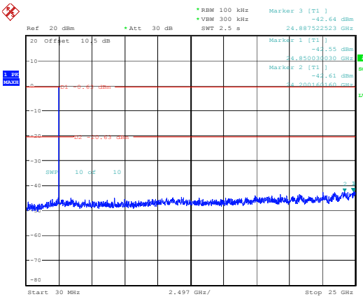
2DH1_High
