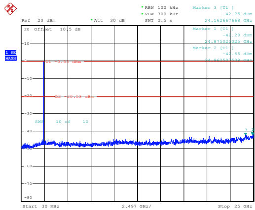
DH1_Low
