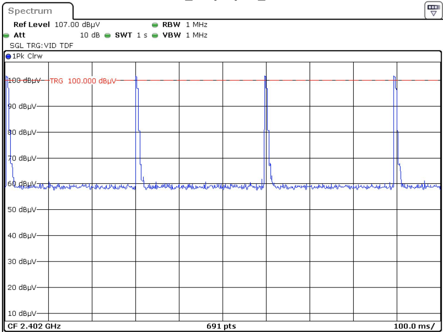
BT_Duty Cycle_1s
