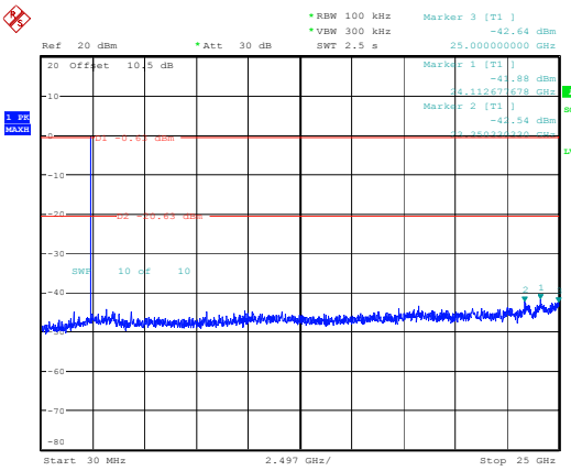
2DH1_Low
