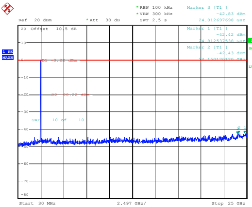
DH1_Middle
