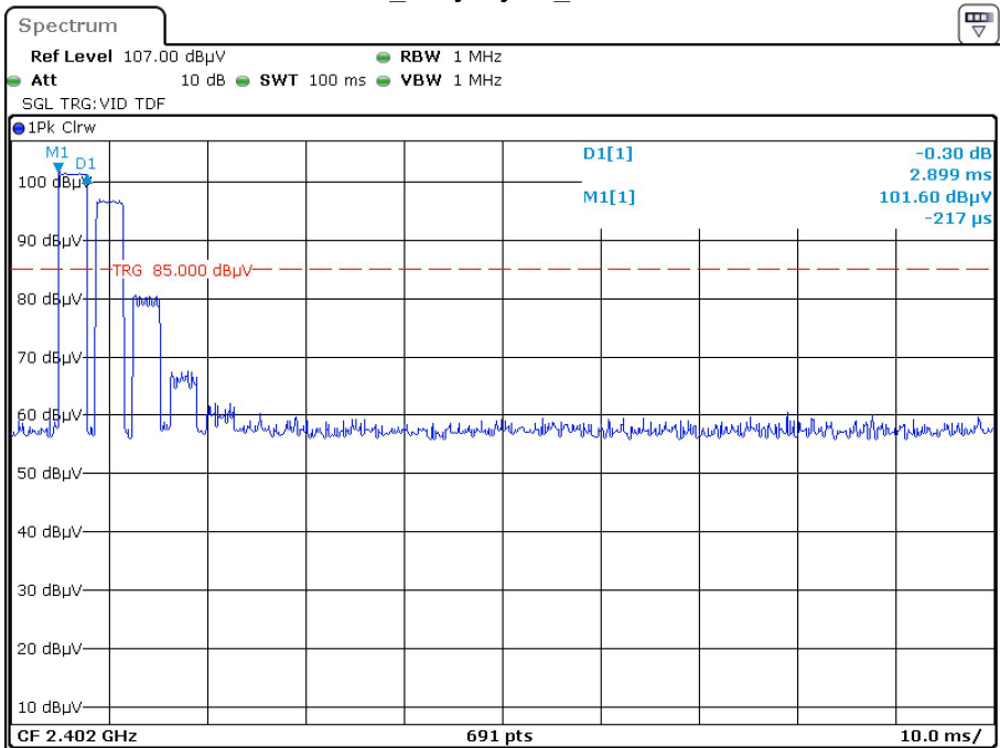
BT_Duty Cycle_100ms
