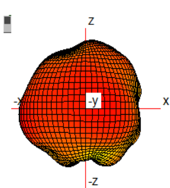
3D Antenna Pattern
