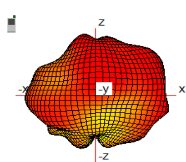
3D Antenna Pattern
