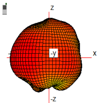
3D Antenna Pattern
