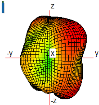
3D Antenna pattern
