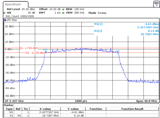
802.11ax20_2437MHz_RU_Full_Chain 0
