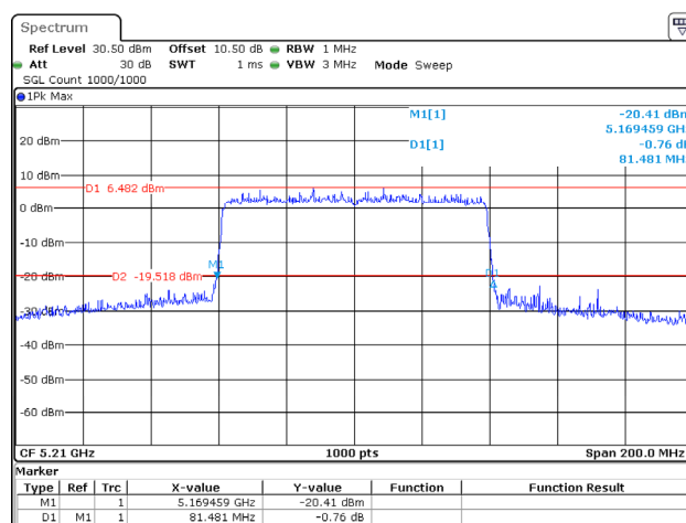
802.11ax80_5210MHz_RU_Full_Chain 1
