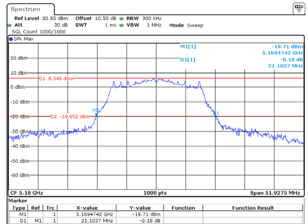
802.11a_5180MHz_Chain 1
