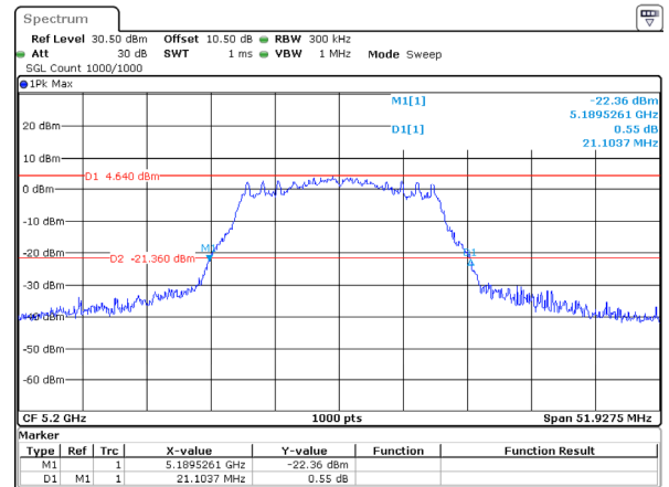
802.11a_5200MHz_Chain 0
