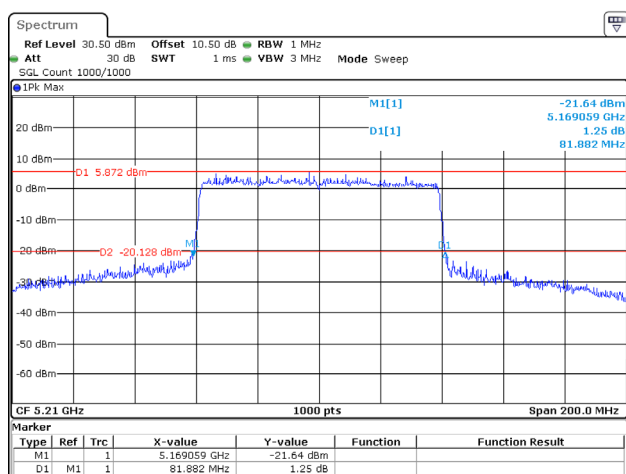
802.11ax80_5210MHz_RU_Full_Chain 0
