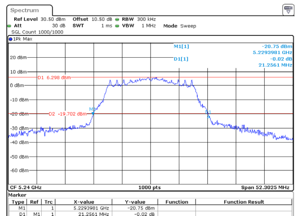
802.11a_5240MHz_Chain 1
