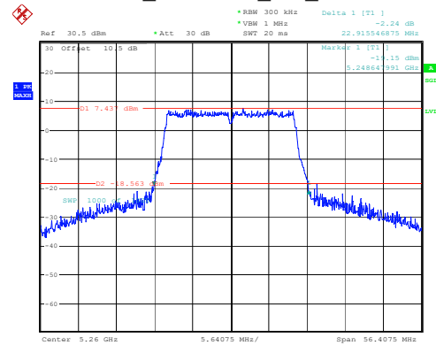
802.11ax20_5260MHz RU_Full 22.916MHz
