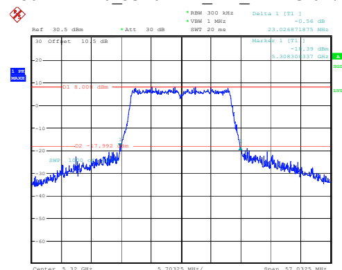
802.11ax20_5320MHz_RU_Full 23.027MHz
