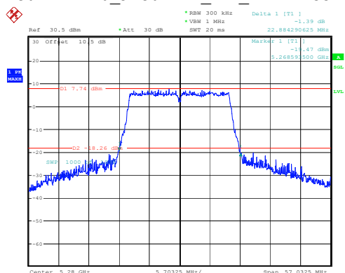
802.11ax20_5280MHz_RU_Full 22.884MHz
