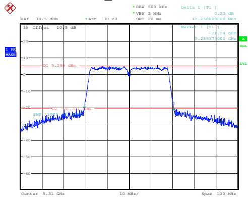
802.11n40_5310MHz 41.250MHz
