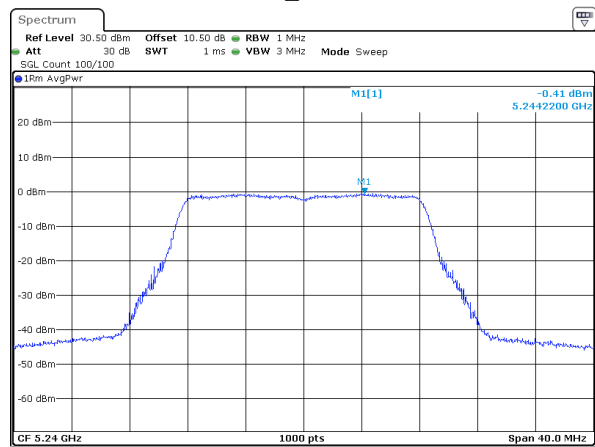
802.11a_5240MHz
