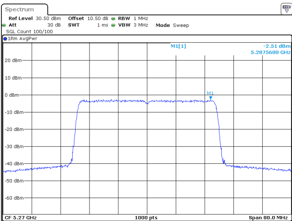
802.11ax40_5270MHz_RU_Full
