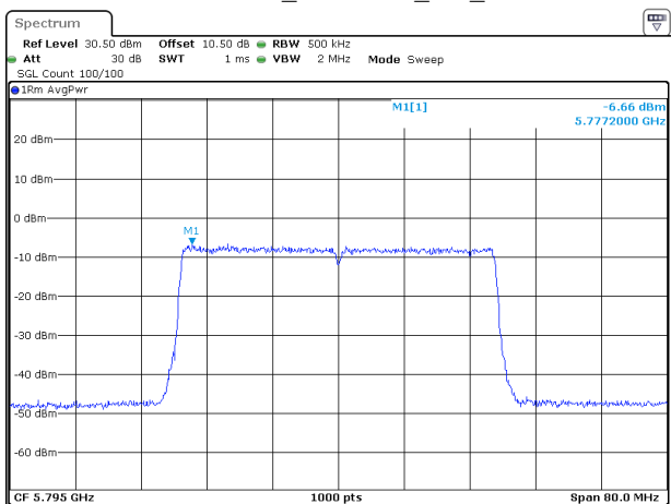
802.11ax40_5795MHz_RU_Full
