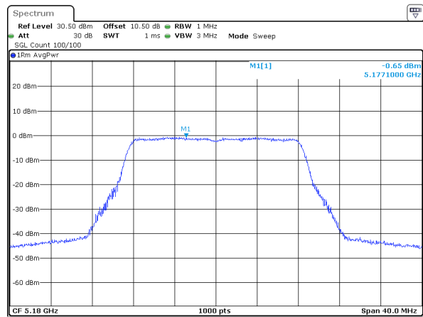
802.11a_5180MHz
