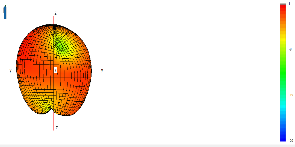
3D Antenna pattern
