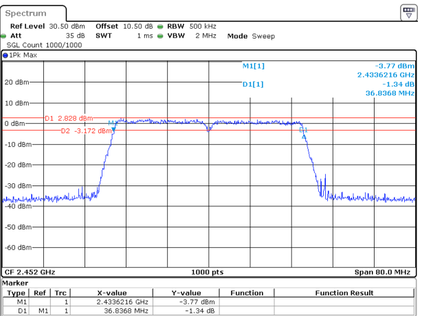
802.11n40_2452MHz
