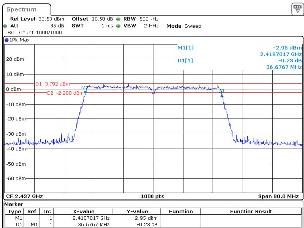
802.11n40_2437MHz
