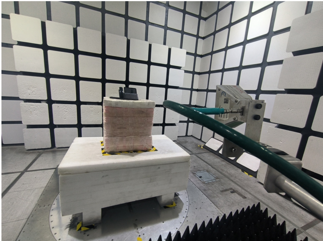
Radiated Emissions View (18-40 GHz)
