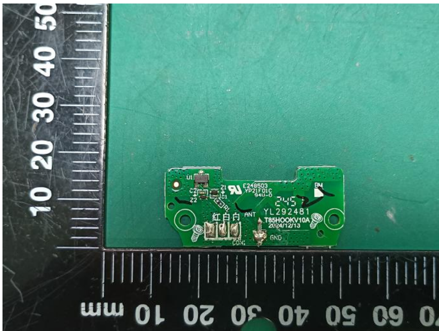
BT/WI-Fi ANT
