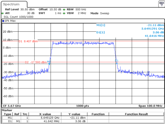
802.11ax40_5670MHz_RU_Full
