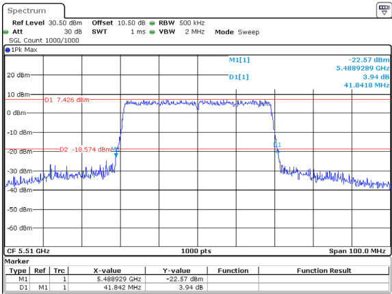
802.11ax40_5510MHz_RU_Full
