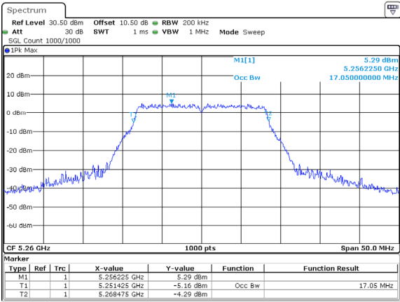
802.11a_5260MHz
