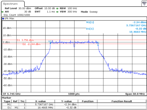
802.11a_5745MHz
