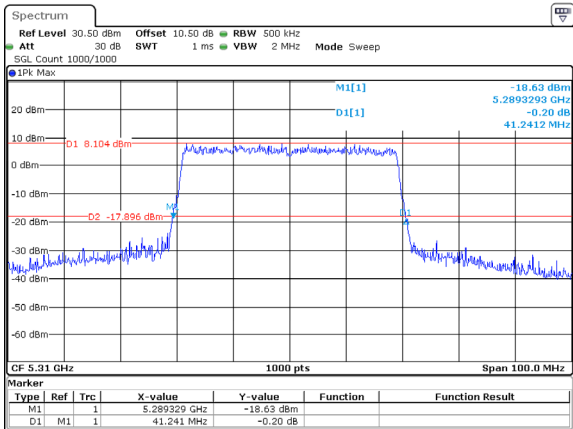
802.11ax40_5310MHz_RU_Full
