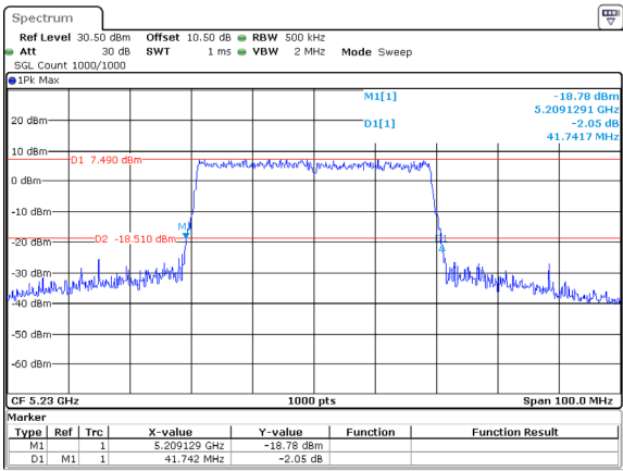
802.11ax40_5230MHz_RU_Full
