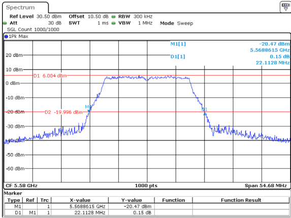
802.11a_5580MHz
