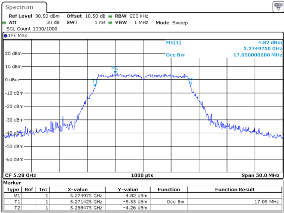
802.11a_5280MHz
