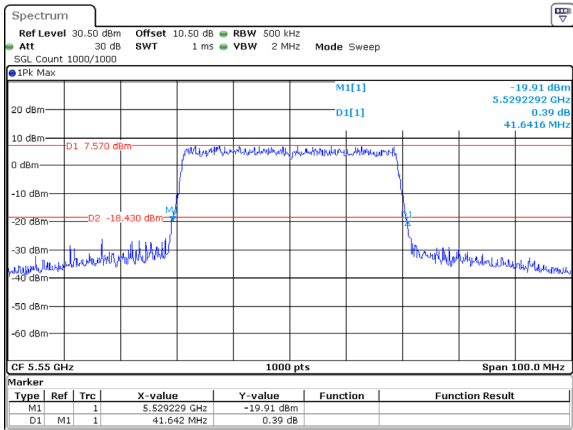
802.11ax40_5550MHz_RU_Full
