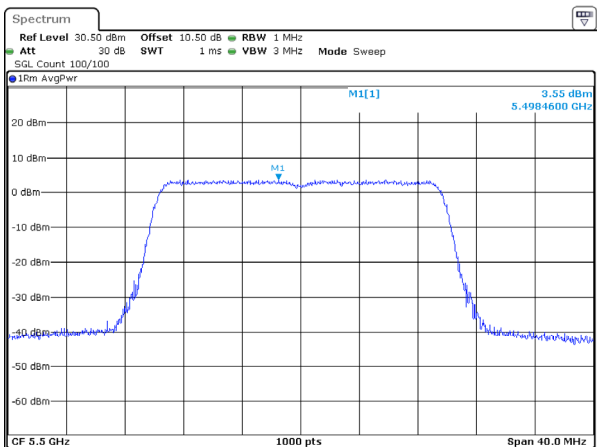
802.11ax20_5500MHz_RU_Full
