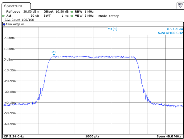
802.11ax20_5240MHz_RU_Full
