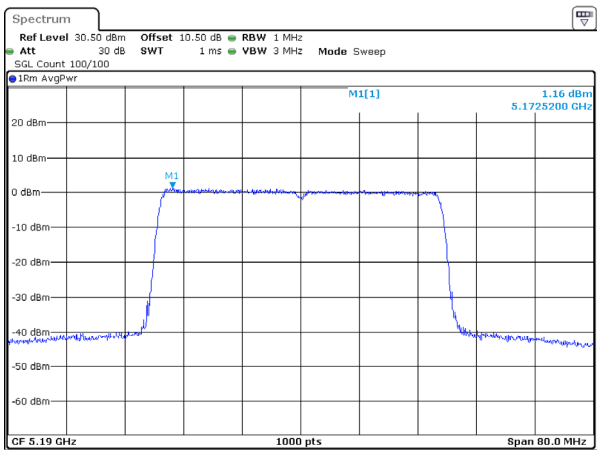
802.11ax40_5190MHz_RU_Full
