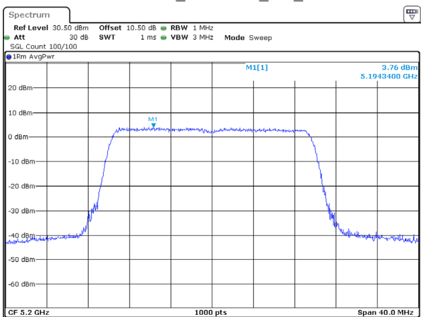
802.11ax20_5200MHz_RU_Full
