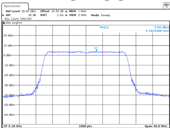
802.11ax20_5180MHz_RU_Full
