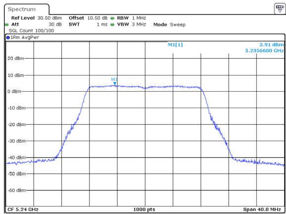
802.11a_5240MHz
