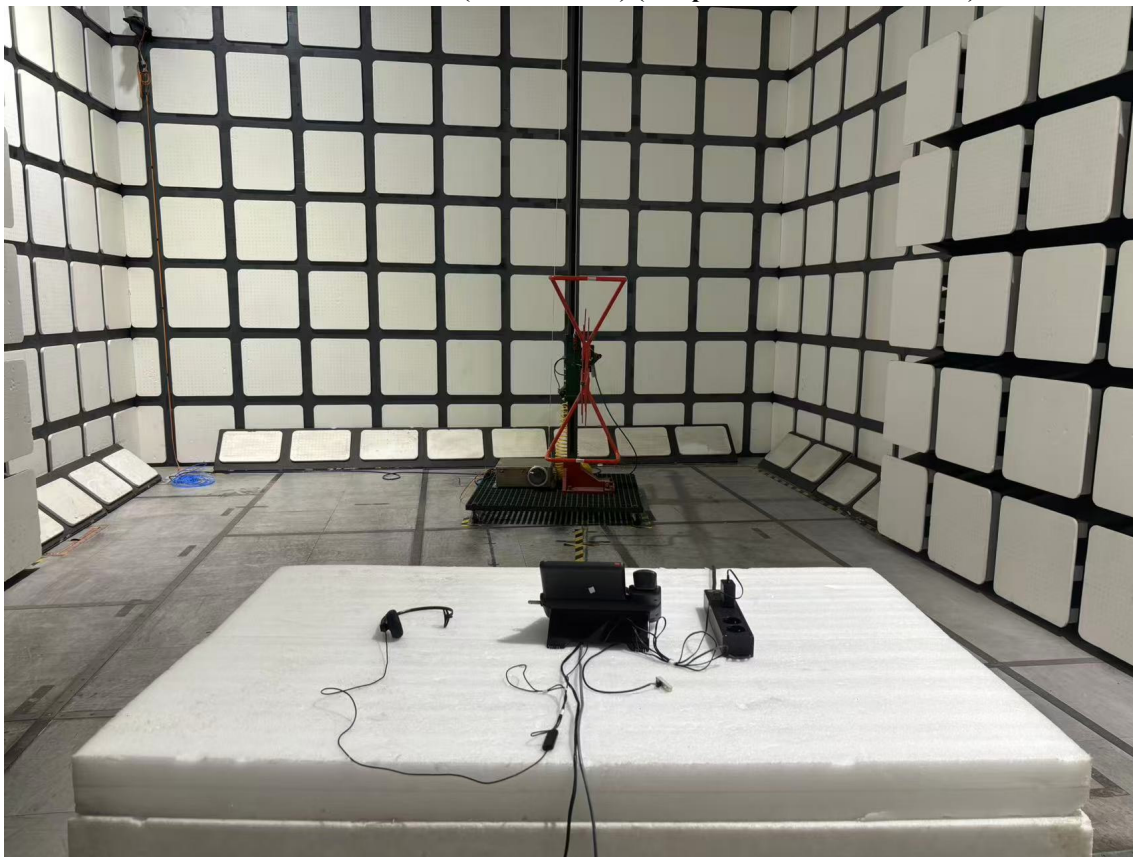
Radiated Emissions View (Below 1 GHz) (Adapter YLPS052000B1-US)
