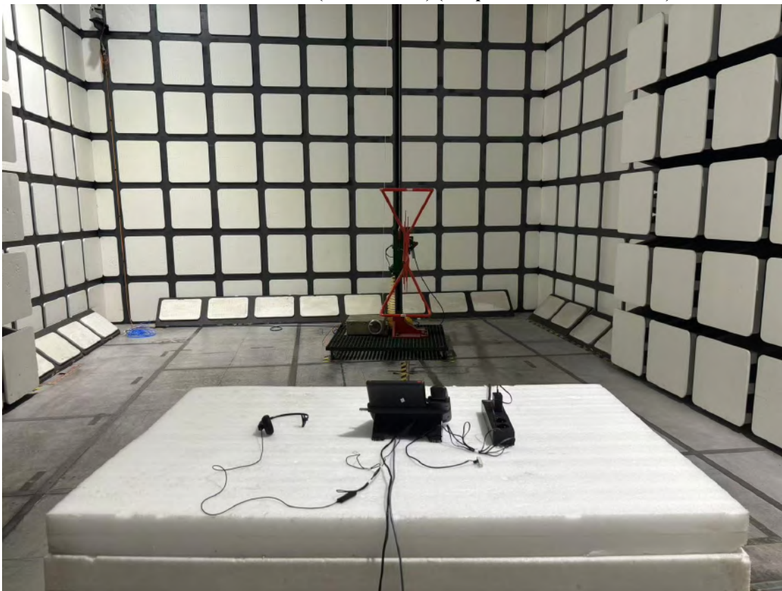
Radiated Emissions View (Below 1 GHz) (Adapter YLPS052000E1-US)
