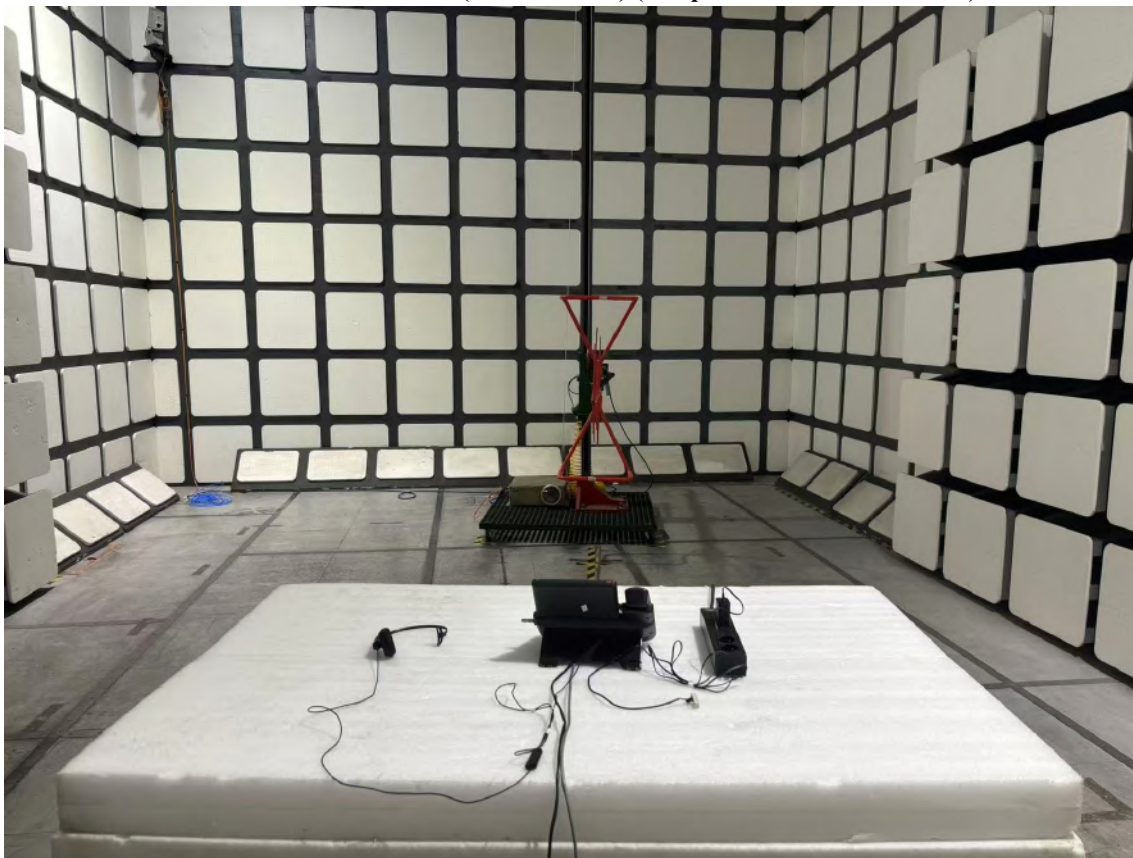
Radiated Emissions View (Below 1 GHz) (Adapter YLPS052000C1-US)
