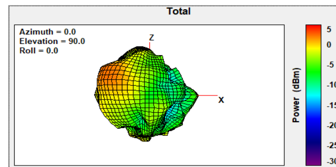
Band4-5.800GHz X-Z PlanarView
