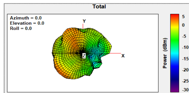
Band4-5.800GHz X-Y Planar View
