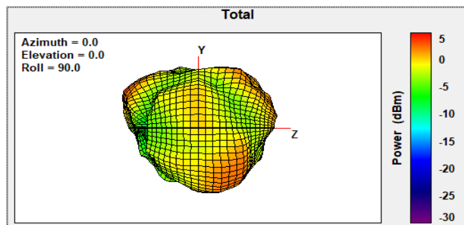
Band4-5.800GHz Y-Z Planar View
