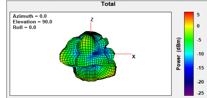
2.44GHz X-Z Planar View
