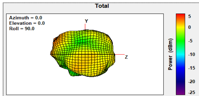
Band1-5.200GHz Y-Z Planar View
