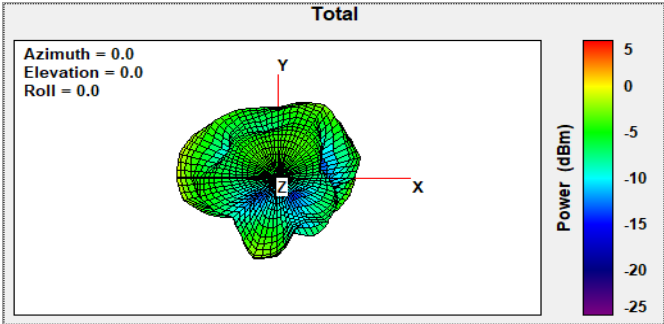
2.44GHz X-Y Planar View
