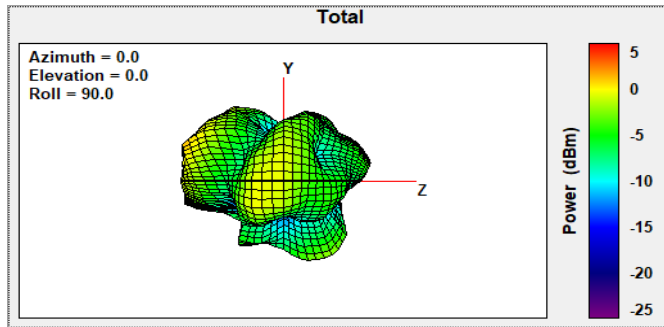
2.44GHz Y-Z Planar View
