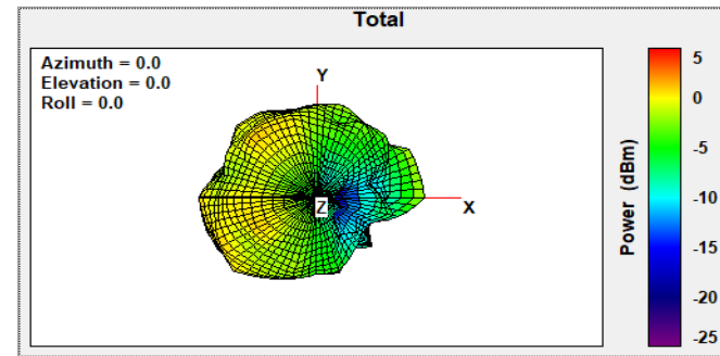
Band1-5.200GHz X-Y Planar View
