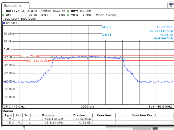
802.11g_2442MHz_Chain 1
