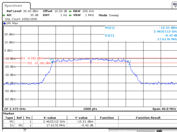
802.11n20_2472MHz_Chain 0
