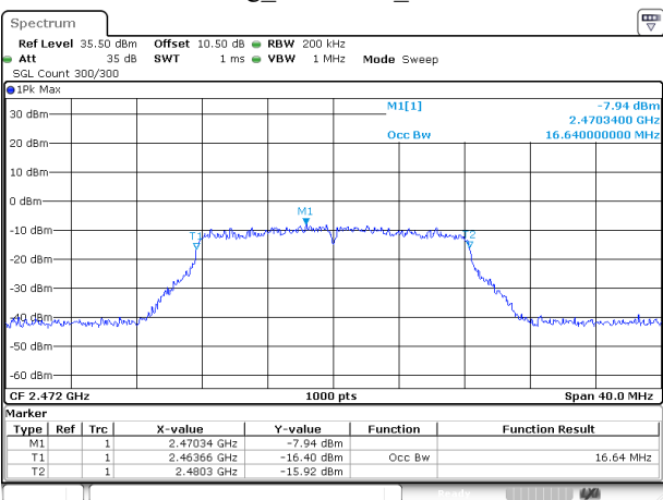
802.11g_2472MHz_Chain 1
