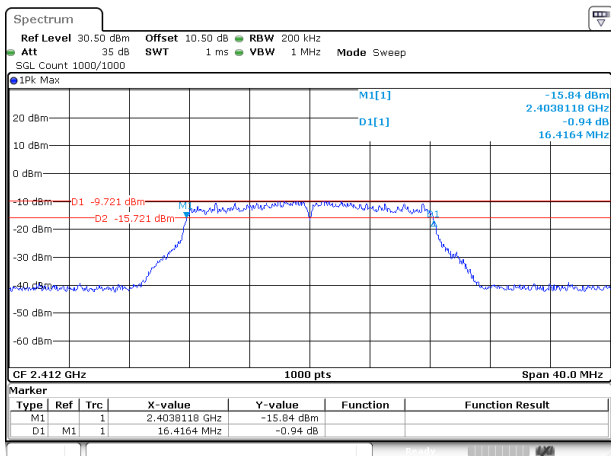
802.11g_2412MHz_Chain 0
