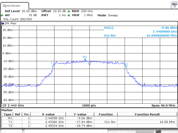
802.11g_2442MHz_Chain 0
