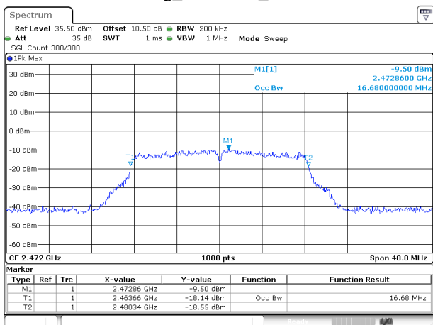
802.11g_2472MHz_Chain 0
