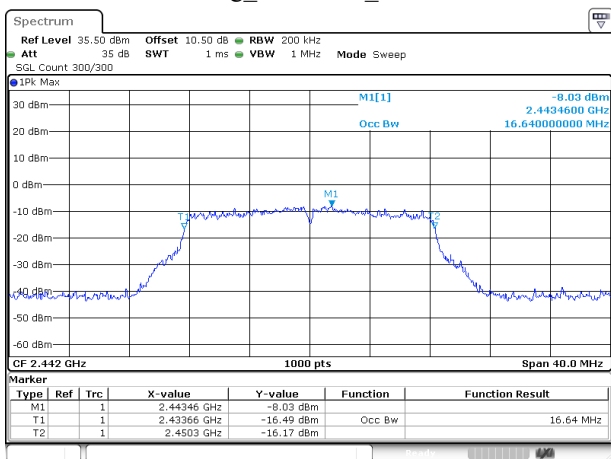
802.11g_2442MHz_Chain 1
