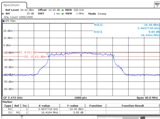
802.11g_2472MHz_Chain 0
