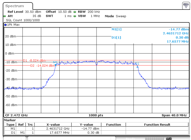
802.11n20_2472MHz_Chain 1
