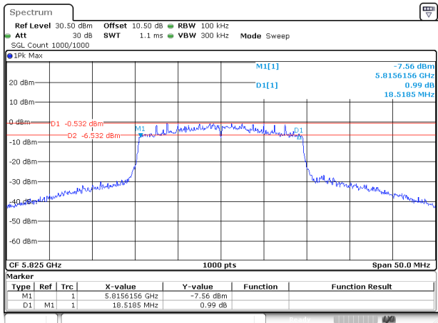
802.11ax20_5825MHz_RU_Full_Chain 0
