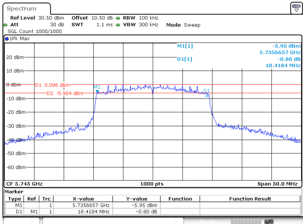
802.11ax20_5745MHz_RU_Full_Chain 0
