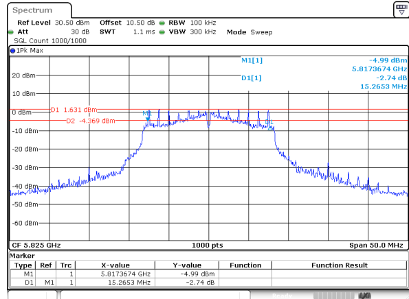
802.11a_5825MHz_Chain 0
