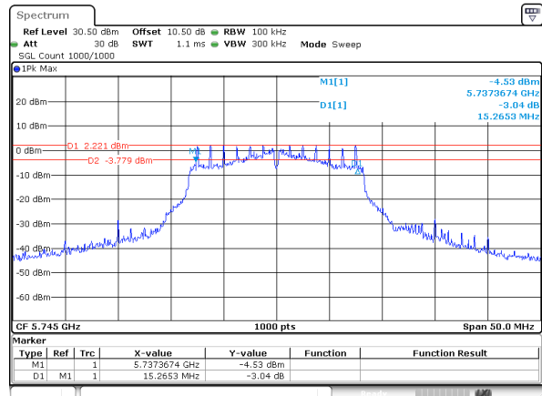
802.11a_5745MHz_Chain 0
