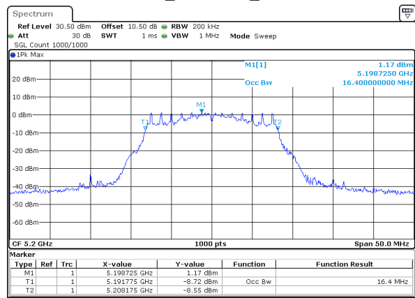
802.11a_5200MHz_Chain 1
