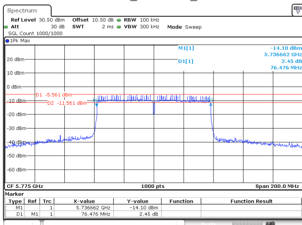
802.11ac80_5775MHz_Chain 1
