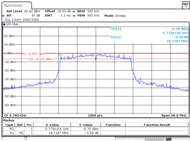
802.11ax20_5785MHz_RU_Full_Chain 1
