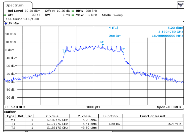
802.11a_5180MHz_Chain 0
