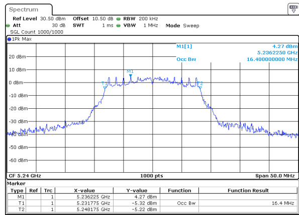
802.11a_5240MHz_Chain 0
