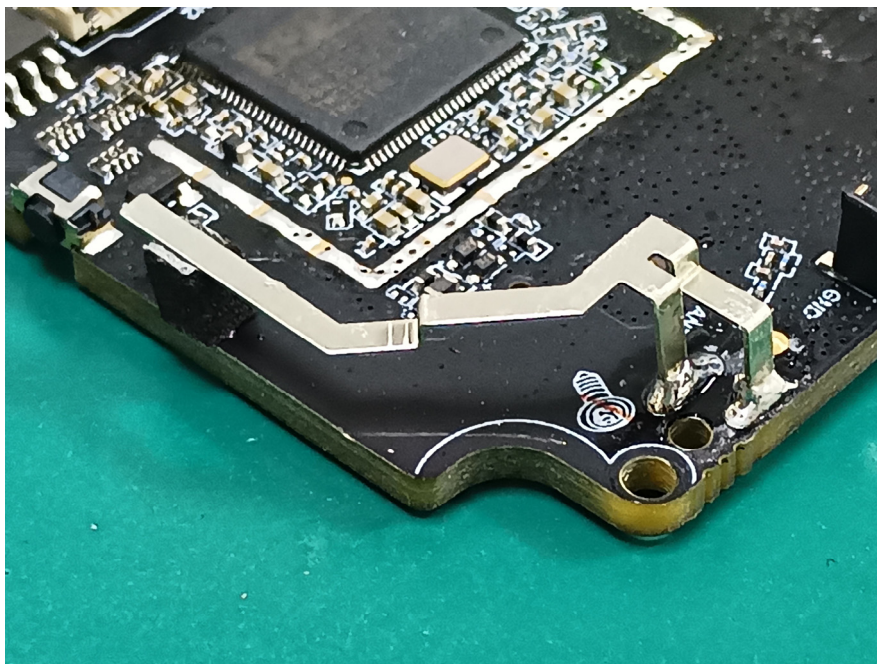
DECT ANT 0
