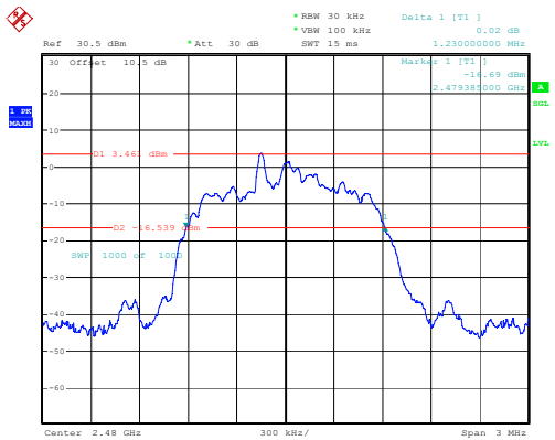
2DH1_High 1.230MHz
