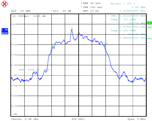
2DH1_High 1.151MHz
