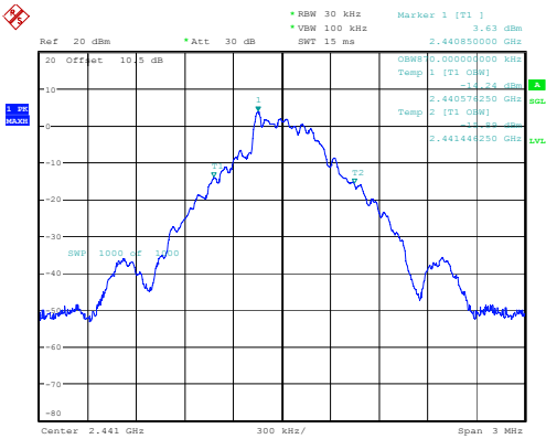
DH1_Middle 0.870MHz
