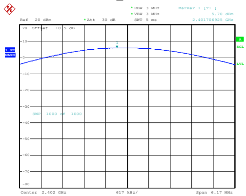
2DH1_Low 5.70dBm
