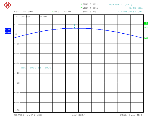
3DH1_Middle 5.75dBm
