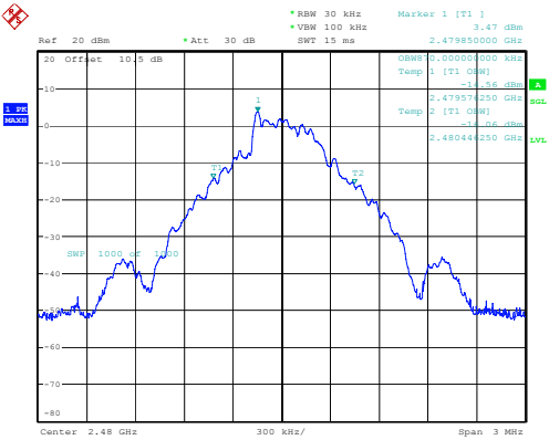
DH1_High 0.870MHz
