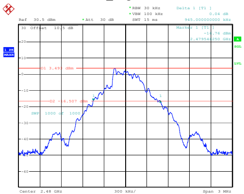
DH1_High 0.945MHz
