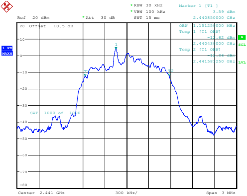
2DH1_Middle 1.151MHz
