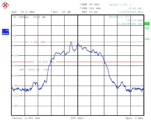
2DH1_Middle 1.234MHz
