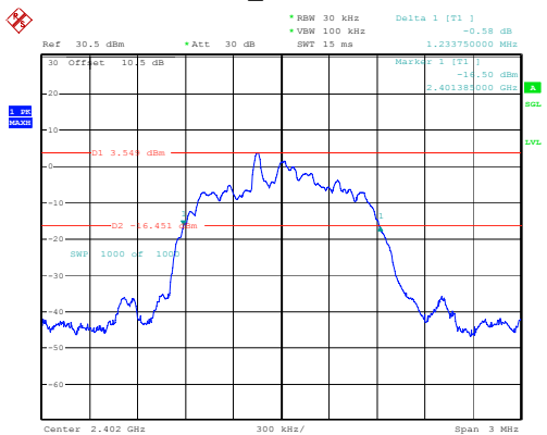
2DH1_Low 1.234MHz
