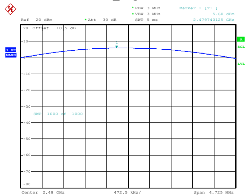
DH1_High 5.60dBm
