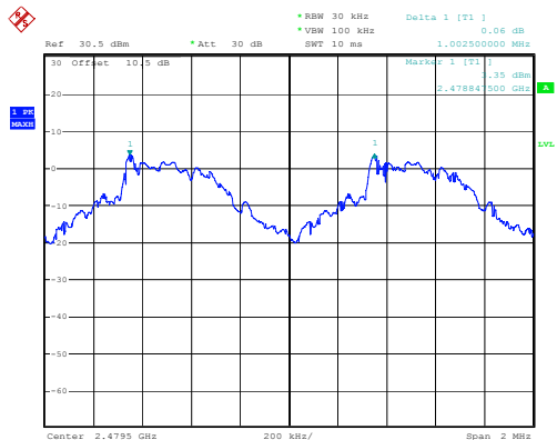
DH1_High 1.003MHz
