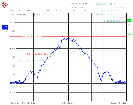
DH1_Low 0.945MHz
