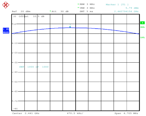
DH1_Middle 5.79dBm
