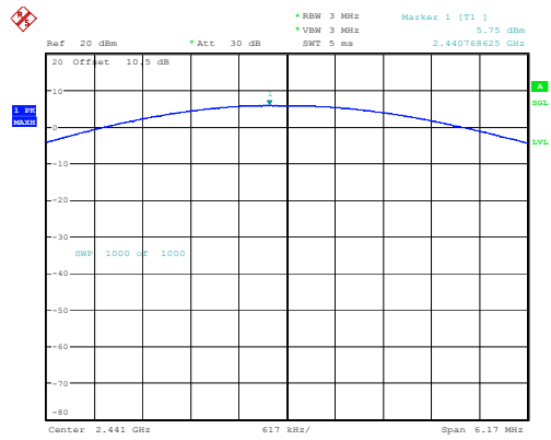
2DH1_Middle 5.75dBm
