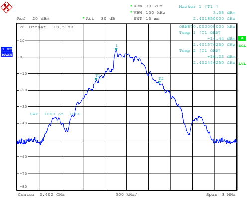
DH1_Low 0.870MHz
