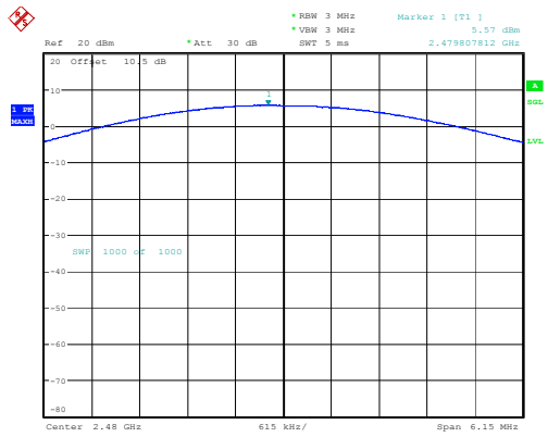
2DH1_High 5.57dBm
