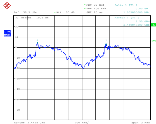
DH1_Middle 1.005MHz
