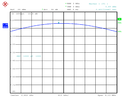
3DH1_Low 5.69dBm
