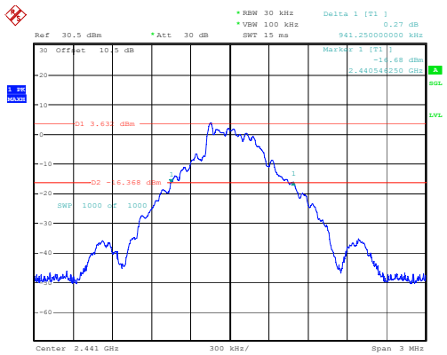
DH1_Middle 0.941MHz
