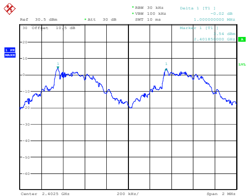
DH1_Low 1MHz
