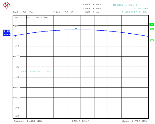
DH1_Low 5.75dBm
