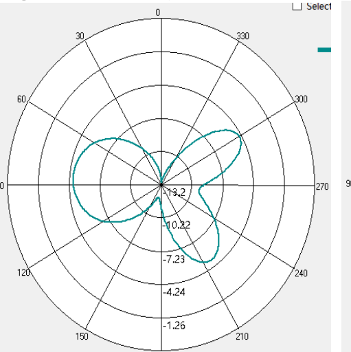
2D Antenna pattern (X->Y;X->Z;Y->Z)
