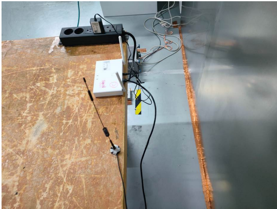
Conducted Emissions - Side View_Adapter 1
