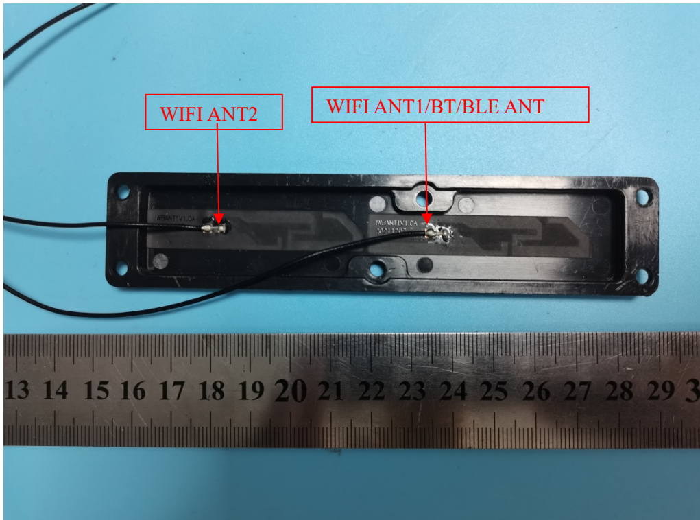
Antenna- iron
