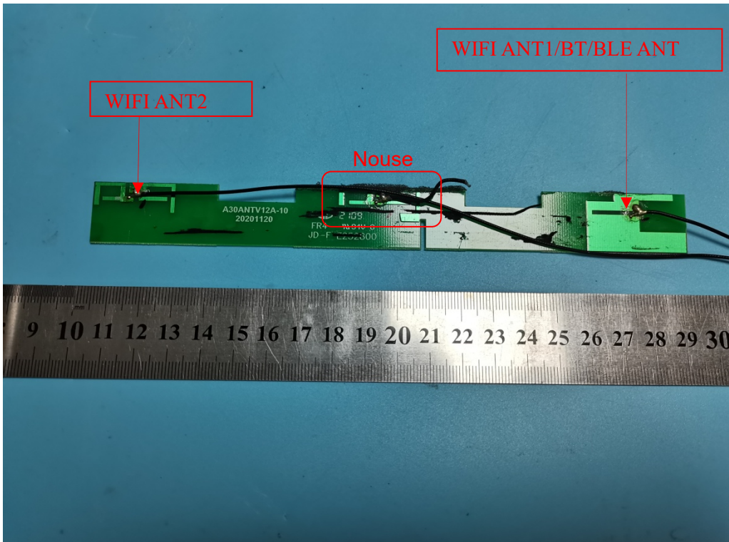
Antenna- PCB
