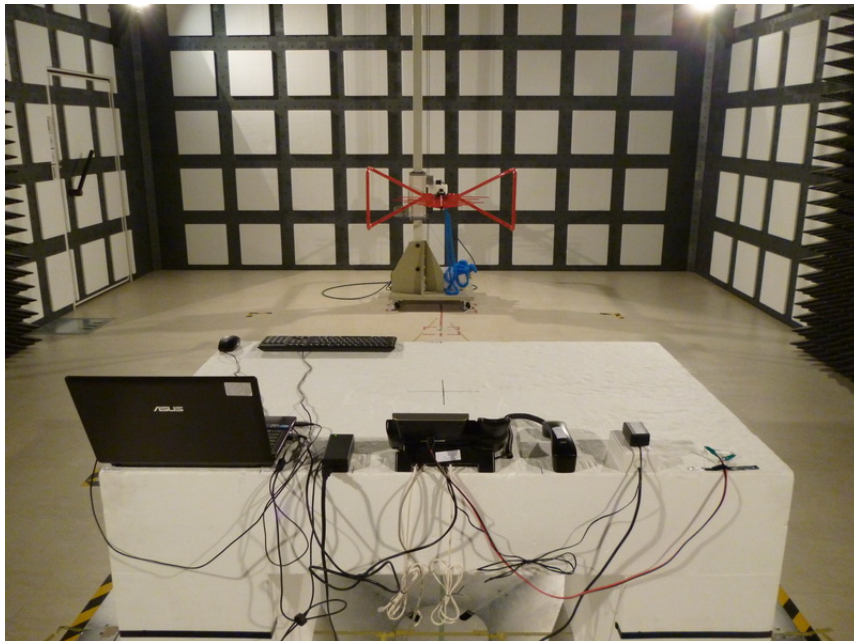
Radiated Emission - Rear View (below 1GHz)
