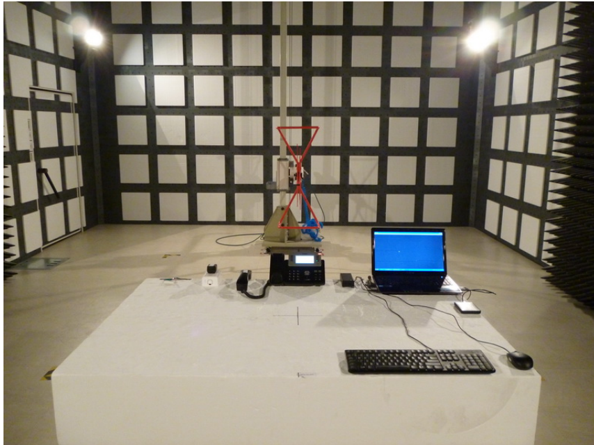
Radiated Emission - Front View (below 1GHz)
