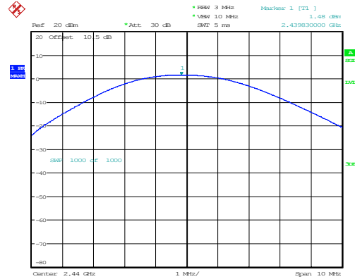
BLE_1M_Middle_Channel
