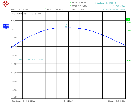
BLE_2M_Middle_Channel
