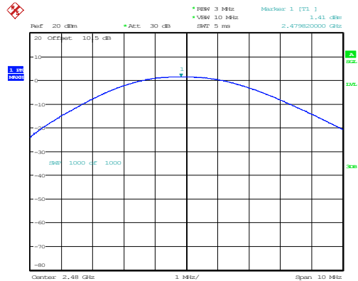
BLE_1M_High_Channel
