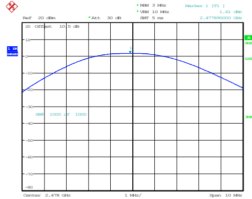
BLE_2M_High_Channel
