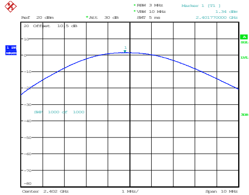
BLE_1M_Low_Channel
