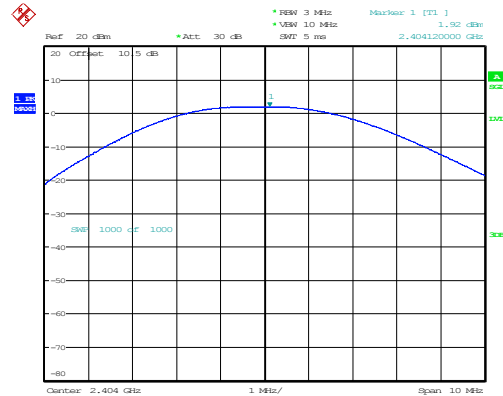
BLE_2M_Low_Channel
