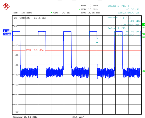
BLE_2M_Middle_Channel
