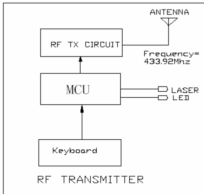
V105 Transmitter Block Diagram
