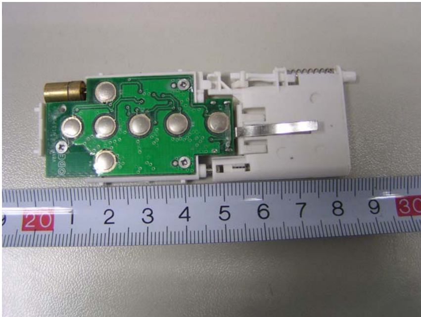
EUT-Inside View (1)
