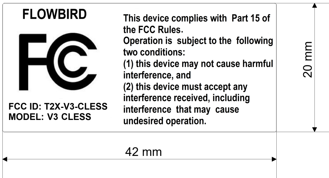
MODELE OF THE FCC ID LABEL
