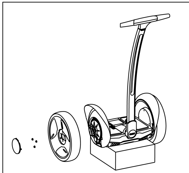
Figure 38: Removing the Tire/Wheel Assembly
