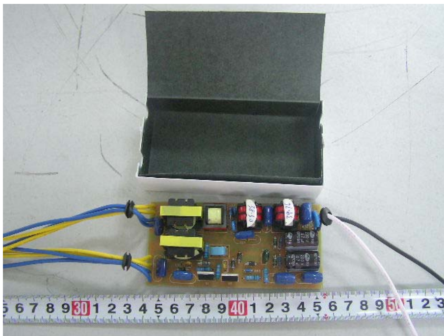
EUT-Inside View
