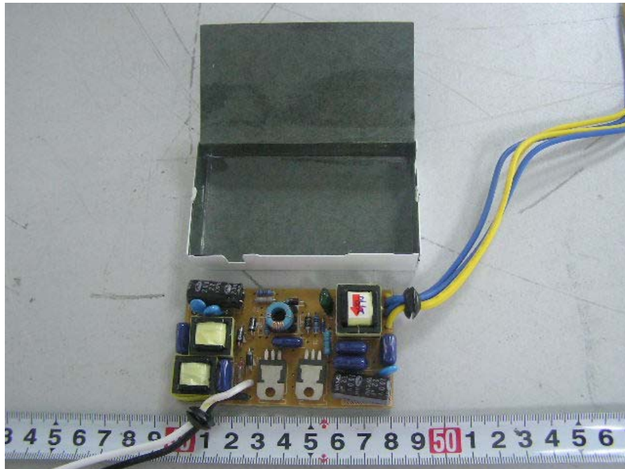
EUT-Inside View
