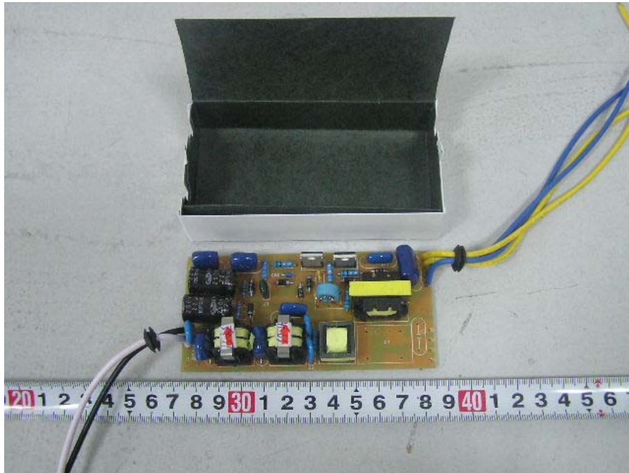
EUT-Inside View
