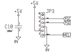
Programming Header
