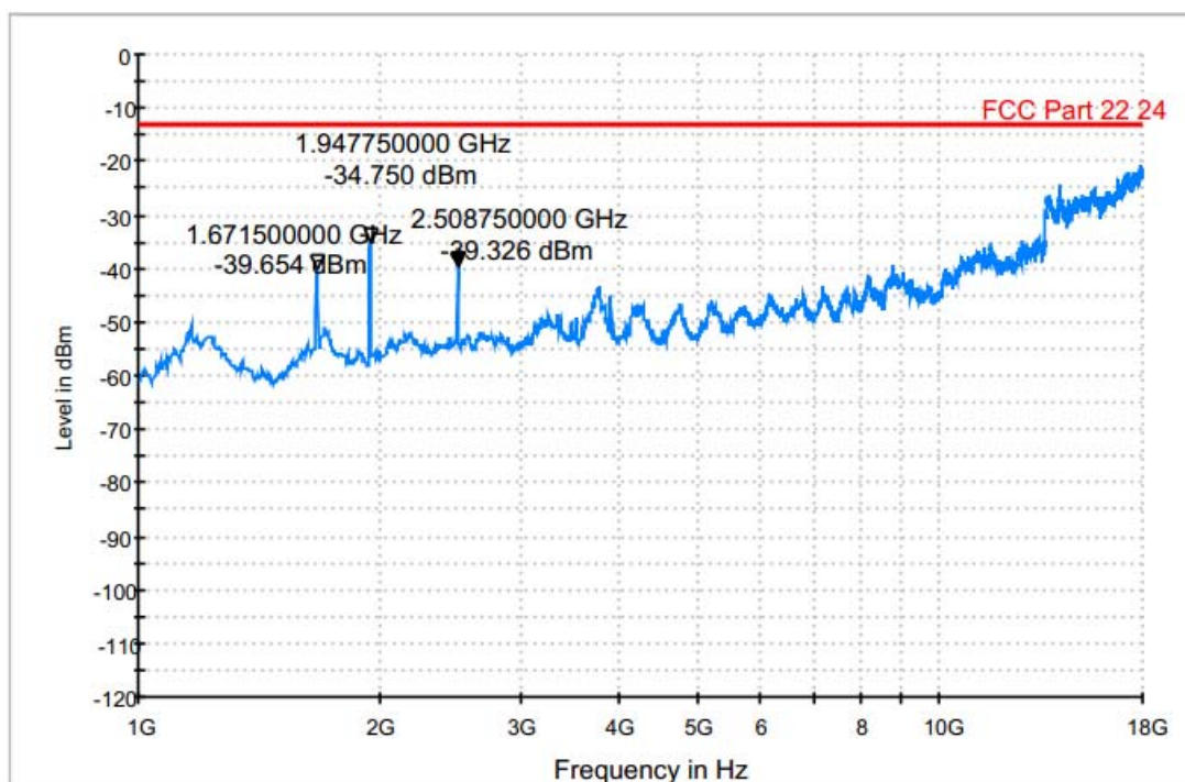
Field Strength of Spurious Radiated 1GHz-18GHz Vertical
