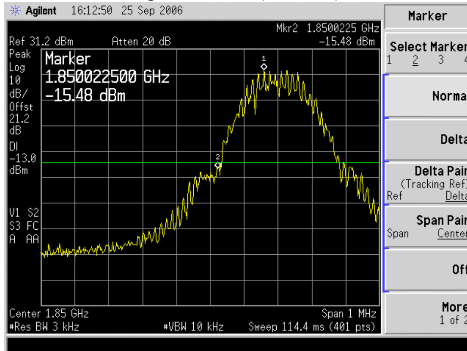
Figure Channel 512 (1850.2MHz)
