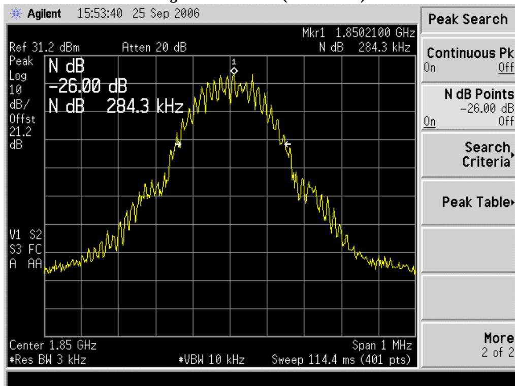
Figure Channel 512(1850.2MHz)
