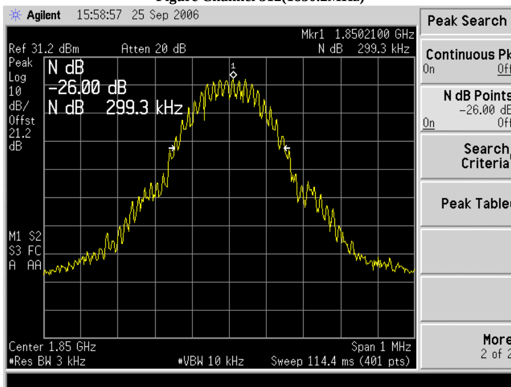
Figure Channel 512(1850.2MHz)
