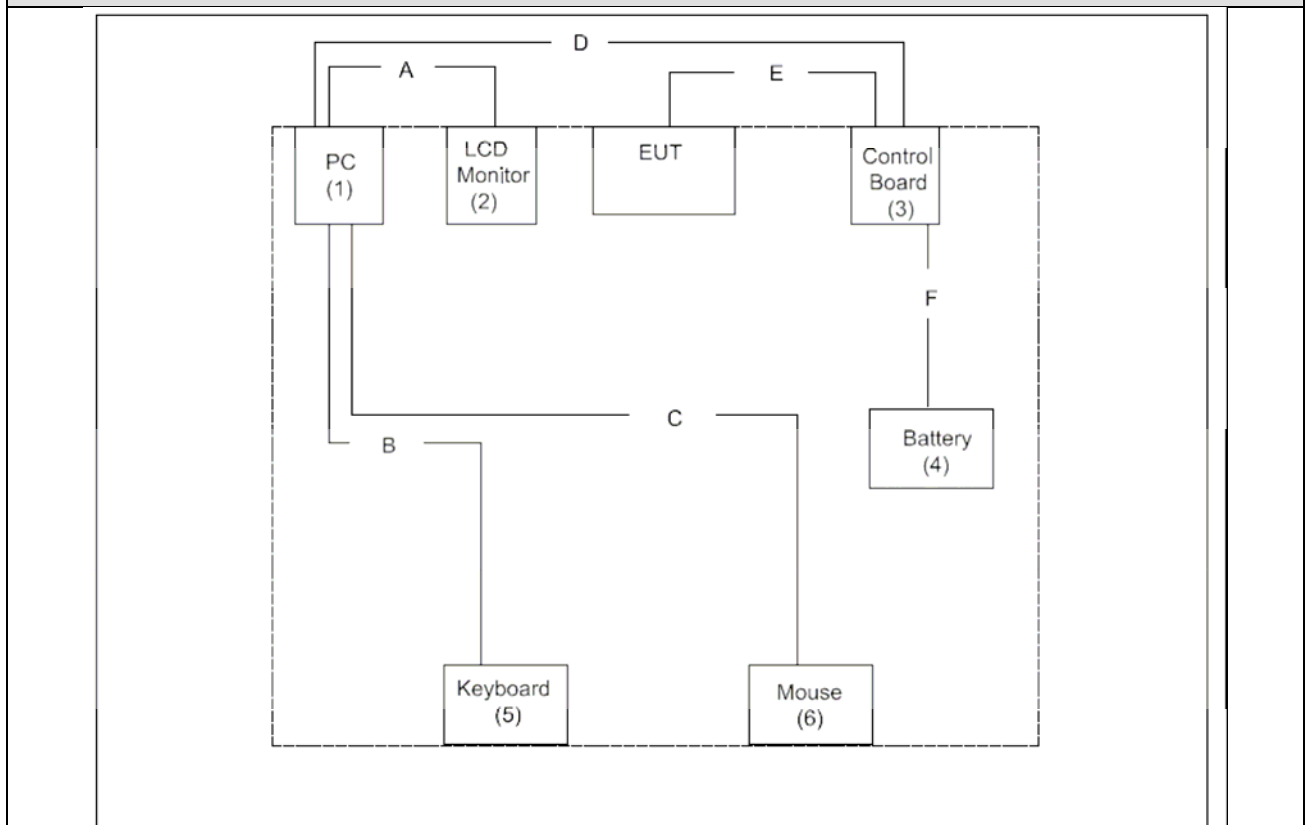
Connection Diagram
