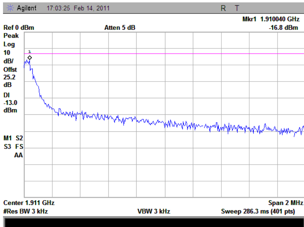
(Plot D: DCS 1900 Channel = 810)
