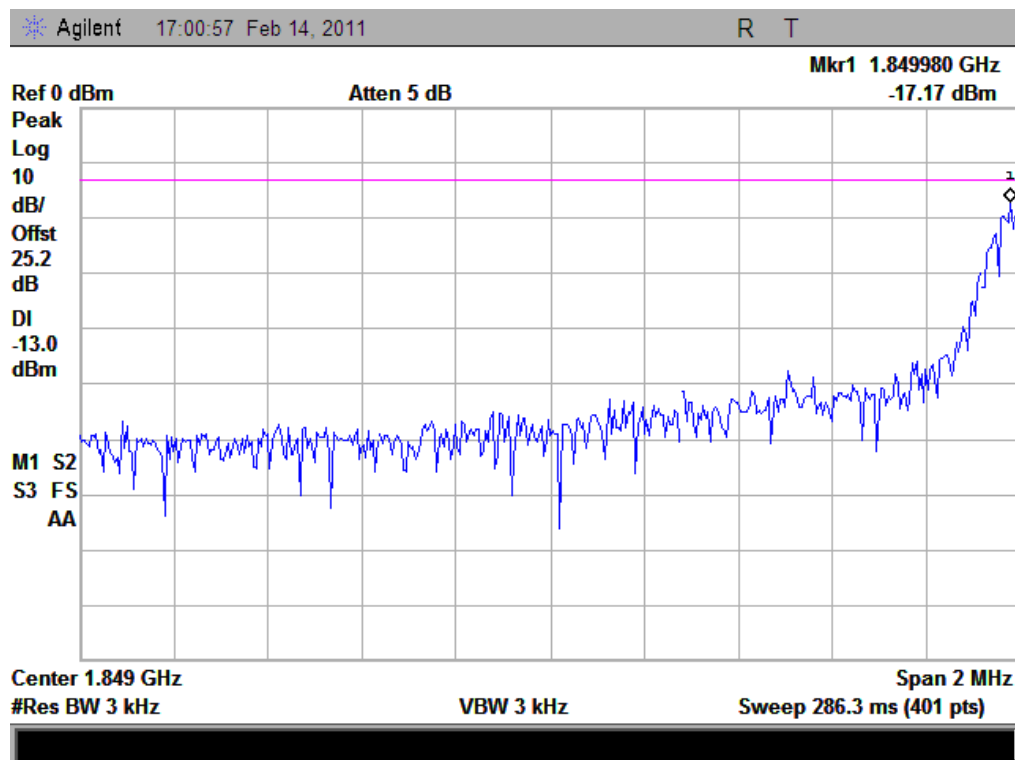
(Plot C: DCS 1900 Channel = 512)
