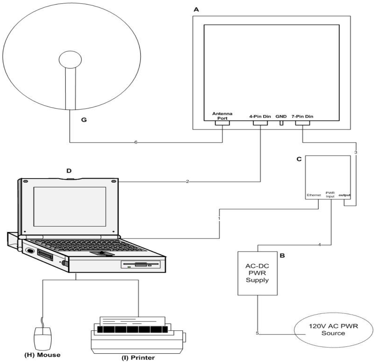
Figure 1. Block Diagram of Test Configuration (Radiated Emissions)
