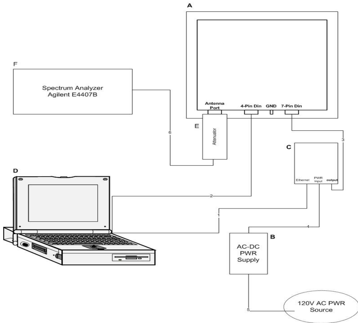
Figure 2. Block Diagram of Test Configuration (Conducted Measurement)
