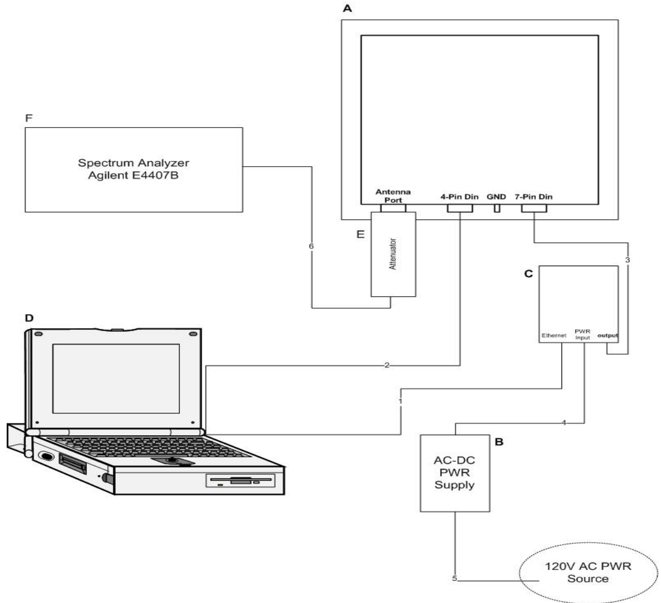
Figure 2. Block Diagram of Test Configuration (Conducted Measurement)
