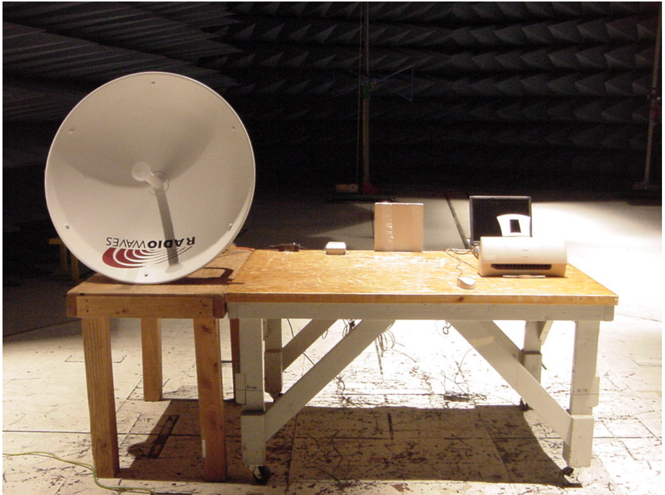
Photograph 5. Radiated Emission Test Setup < 1 GHz
