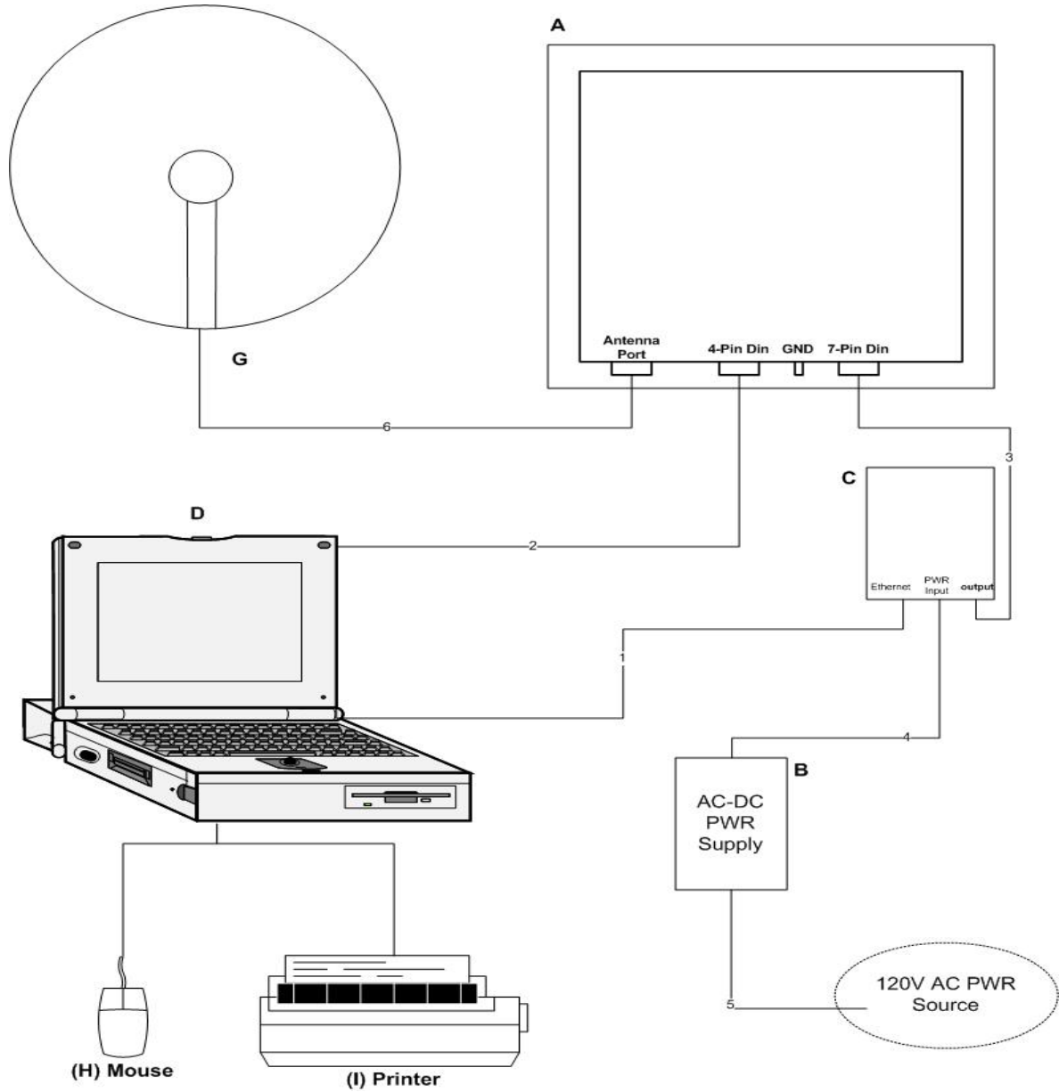
Figure 1. Block Diagram of Test Configuration (Radiated Emissions)
