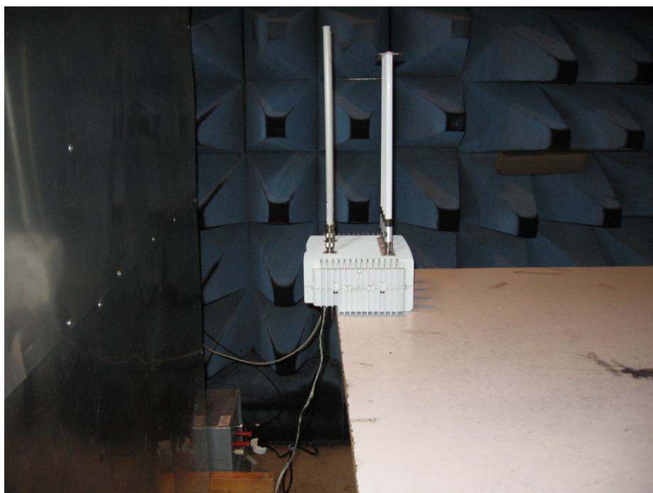
Figure 2. Conducted Emission From AC Mains Test Side
