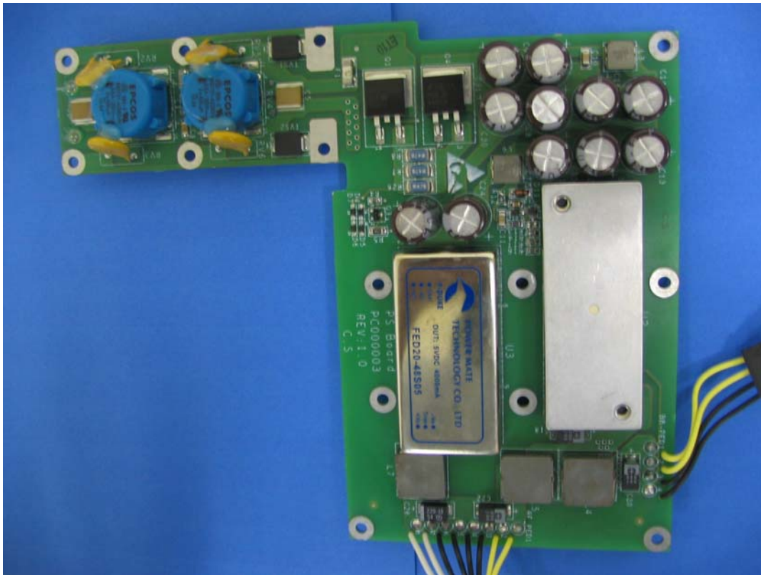
PS board bottom view
