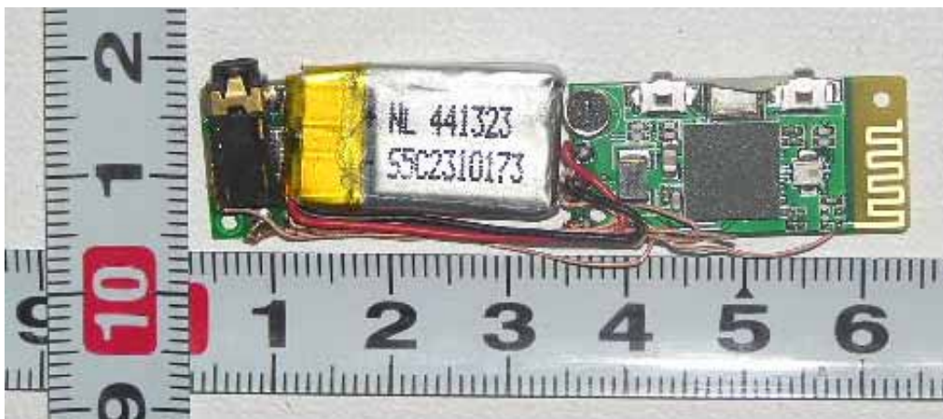
EUT - PCB View (The other Side)
