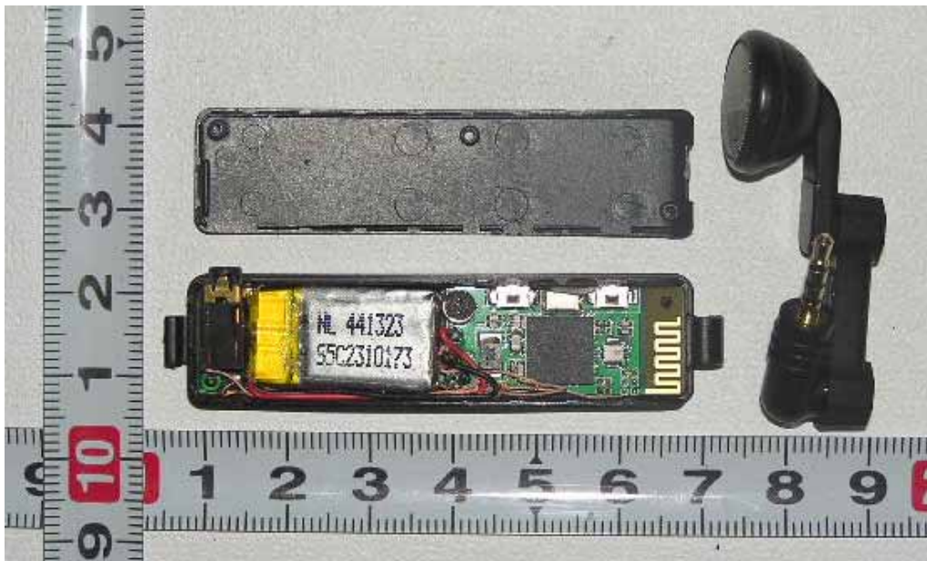
EUT - PCB View (One Side)
