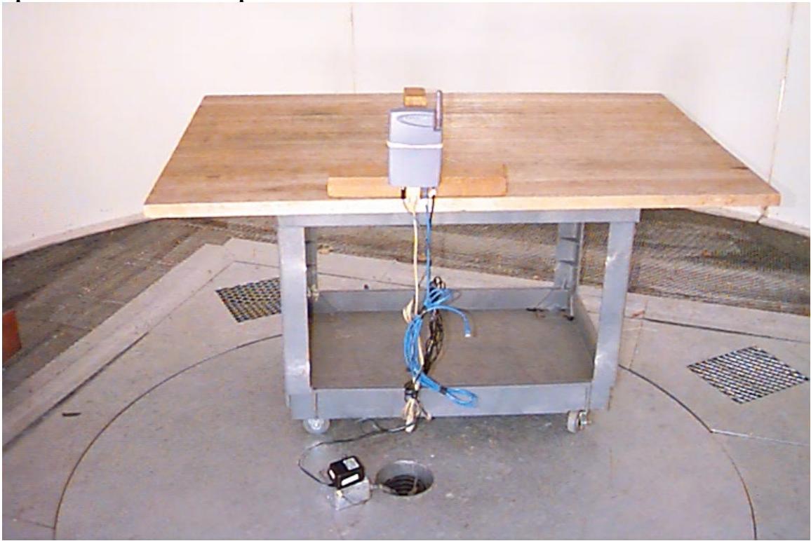
Spurious Emissions Setup:
