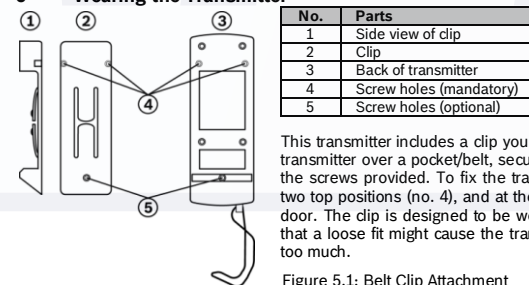
Figure 5.1: Belt Clip Attachment
